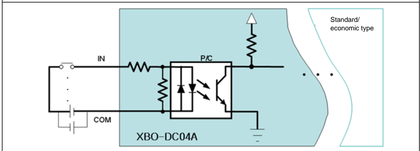
Circuit configuration
