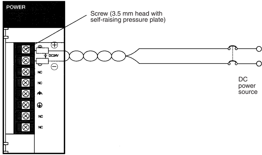
C200HW-PD024/025 Power Supply Unit
