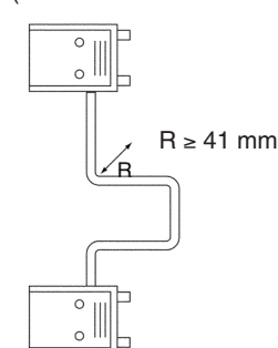
Cables for CS1 Long-distance Expansion Racks (Cable diameter: 10 mm)
