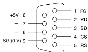
Connector Pin Arrangement for RS-232C Port
