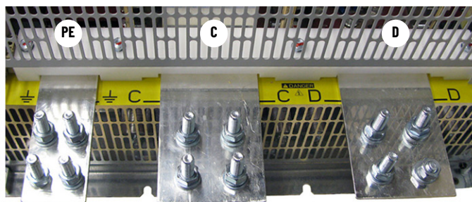
Bottom of Drive
