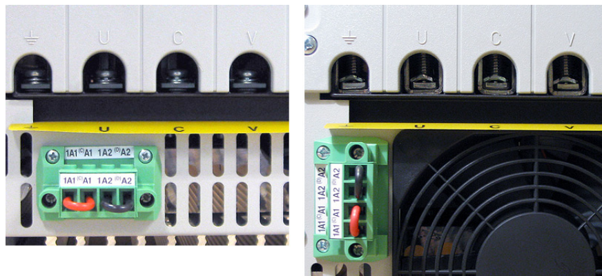
Shown with terminals jumpered for internal armature voltage feedback.
