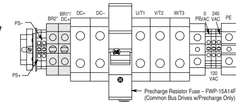
Frame 5 - 100 HP Normal Duty 650V DC Input
