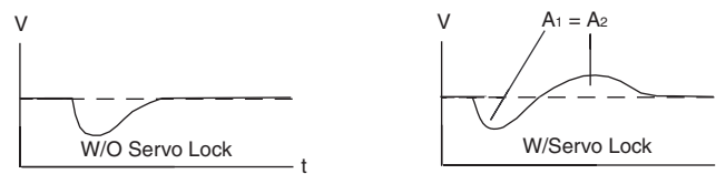
Velocity Response to Step Load
