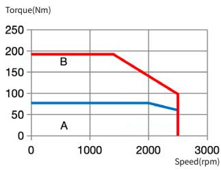
IMS20A-26M41D20C-4-***
