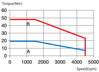
IMS20B-18M75C15C-4-***
