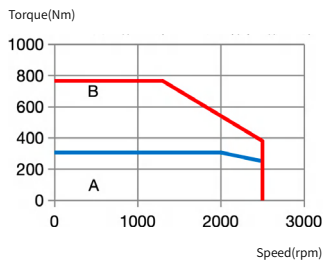
IMS20A-26M64D20C-4-***
