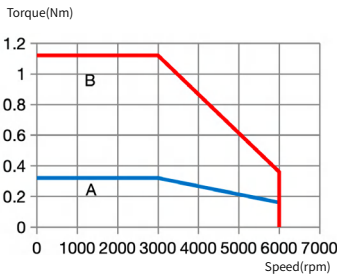
IMS20B-04L10B30C-2-***
