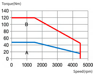
IMS20B-18M75C15C-4-***
