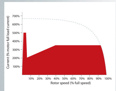
Constant current/ current ramp – shown here with kickstart
