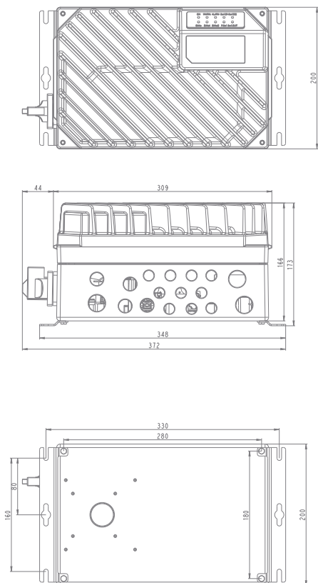
Enclosure size MF1 (0.37 – 2.2 kW/0.5 – 3.0 HP)
