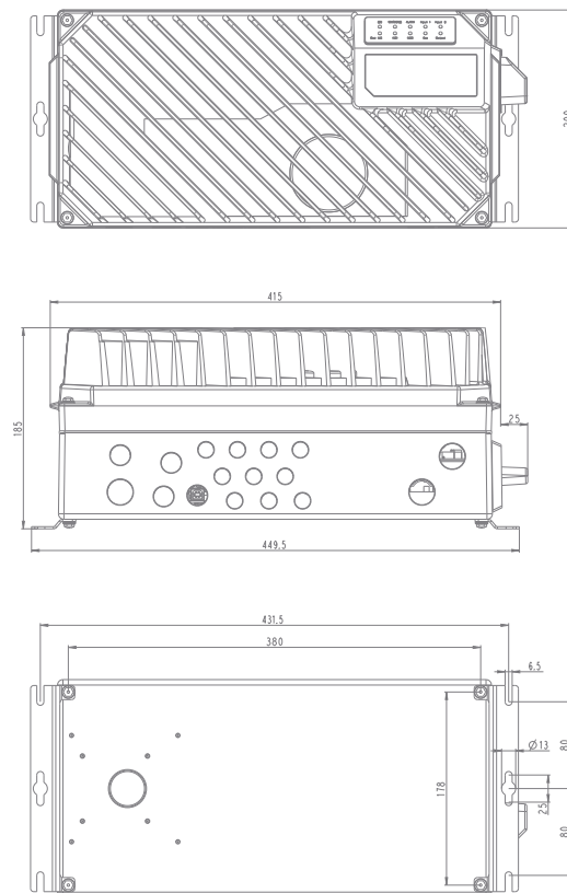
Enclosure size MF2 (0.37 – 3 kW/0.5 – 4.0 HP)
