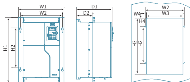
AC 3PH 380V 110~200kW mounting diagram
