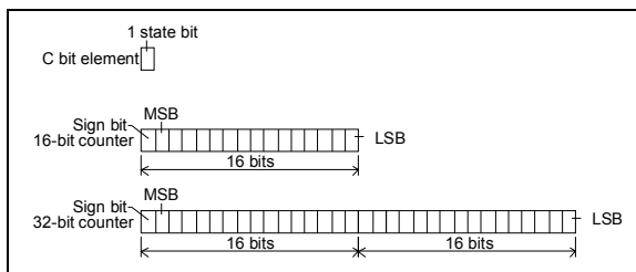
Figure 3-4 C element
