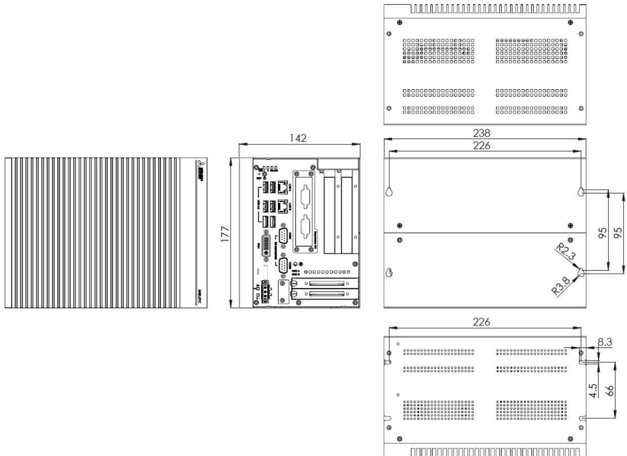
Figure 1.1 MI2012-W Dimensions
