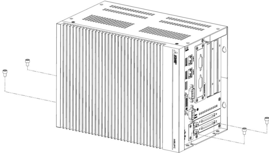
Figure 3.2 Stand Mount
