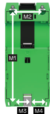
Mounting Dimensions
