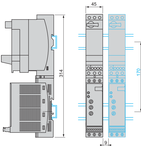
TeSys U combination (non-reversing power base) and ATSU 01N222LT to ATSU 01N232LT Mounting on \perp r (35 mm) rail with VW3 G4104 connector
