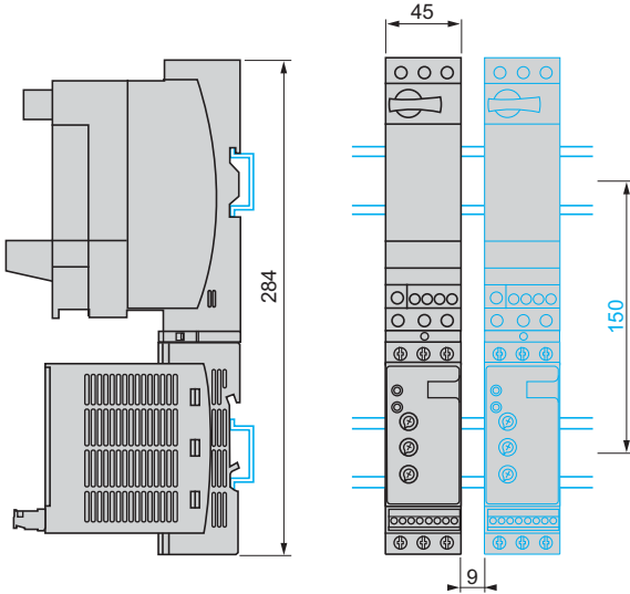
TeSys U combination (non-reversing power base) and ATSU 01N222LT to ATSU 01N232LT Mounting on \perp r (35 mm) rail with VW3 G4104 connector
