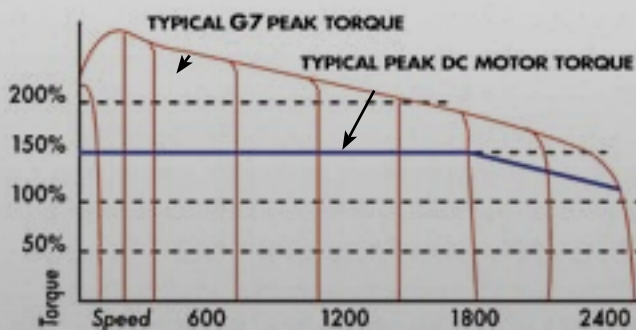
Peak Torque vs Speed (4 Pole Motor)
