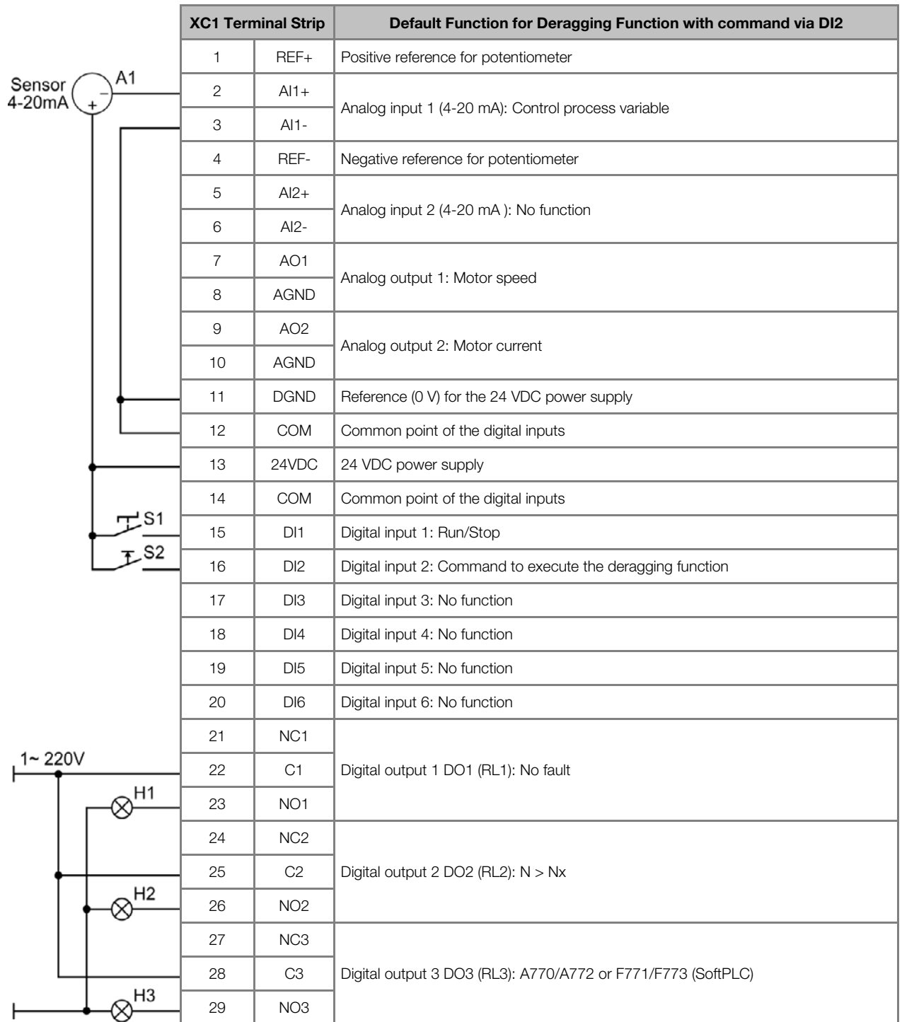
Figure 2.18 – Terminal strip XC1 for deragging function with command via digital input DI2
