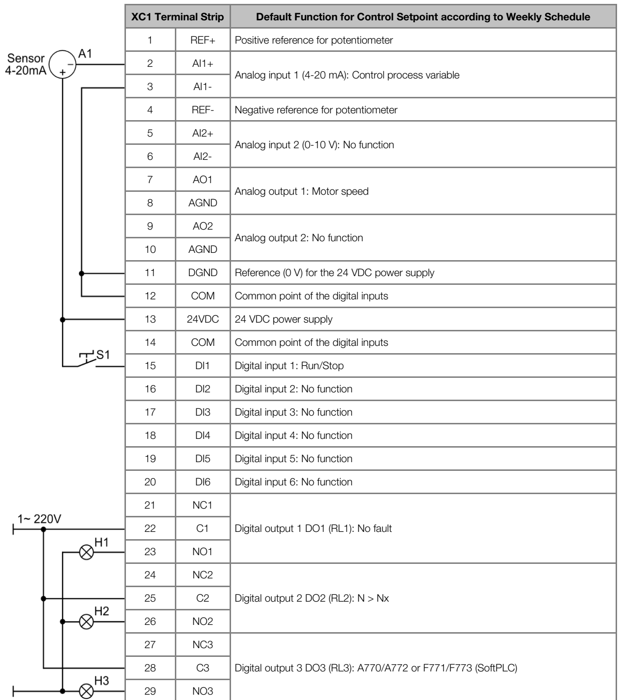
Figure 2.8 – Terminal strip XC1 for control setpoint according to weekly schedule
