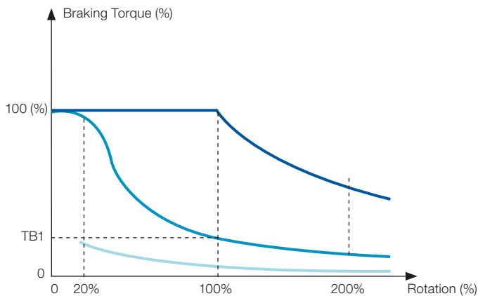
Typical Braking Torque x Speed Graph for a 10 HP / 7.5 kW motor driven by a CFW700
