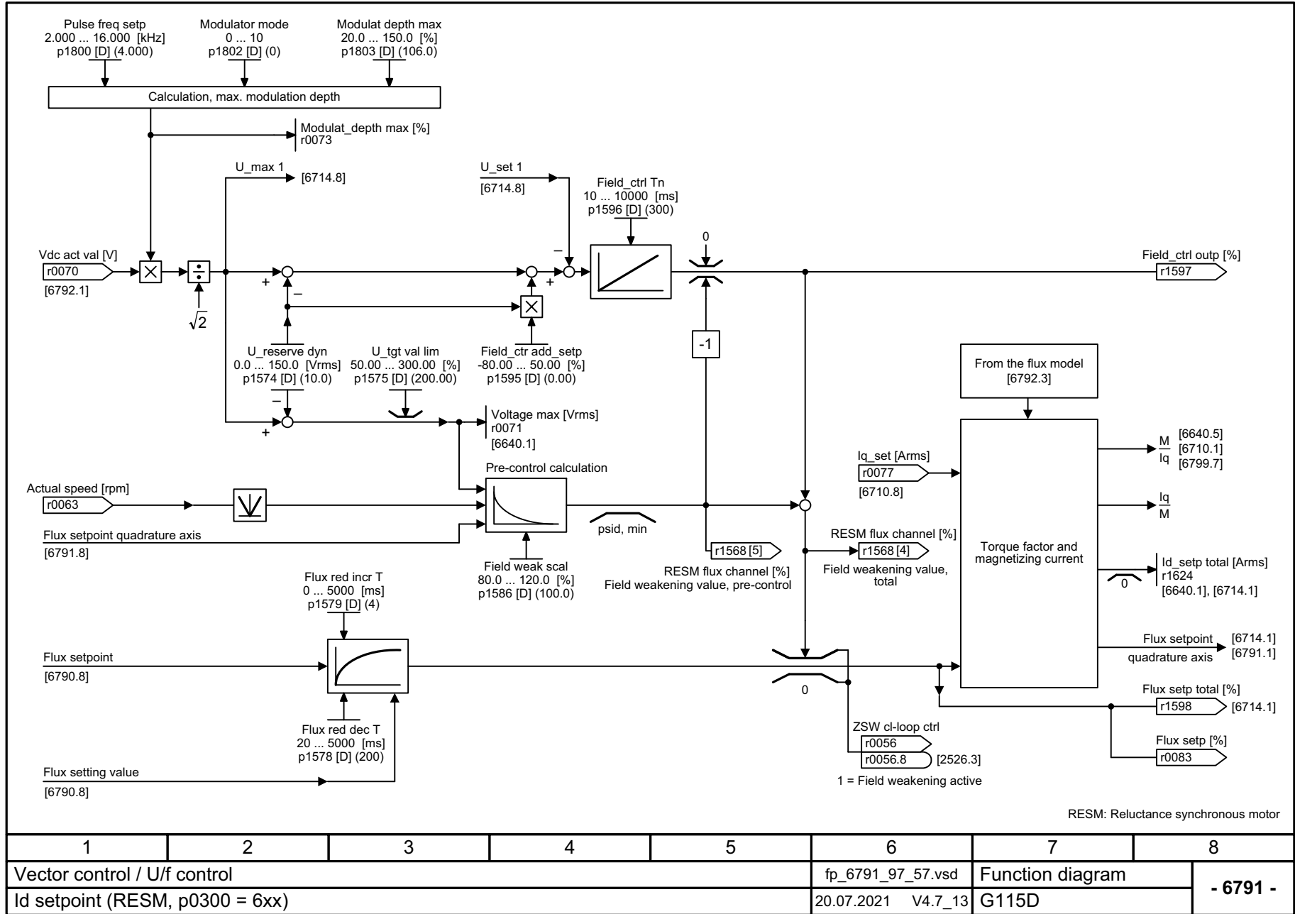
Fig. 3-103 6791 – Id setpoint (RESM, p0300 = 6xx)
