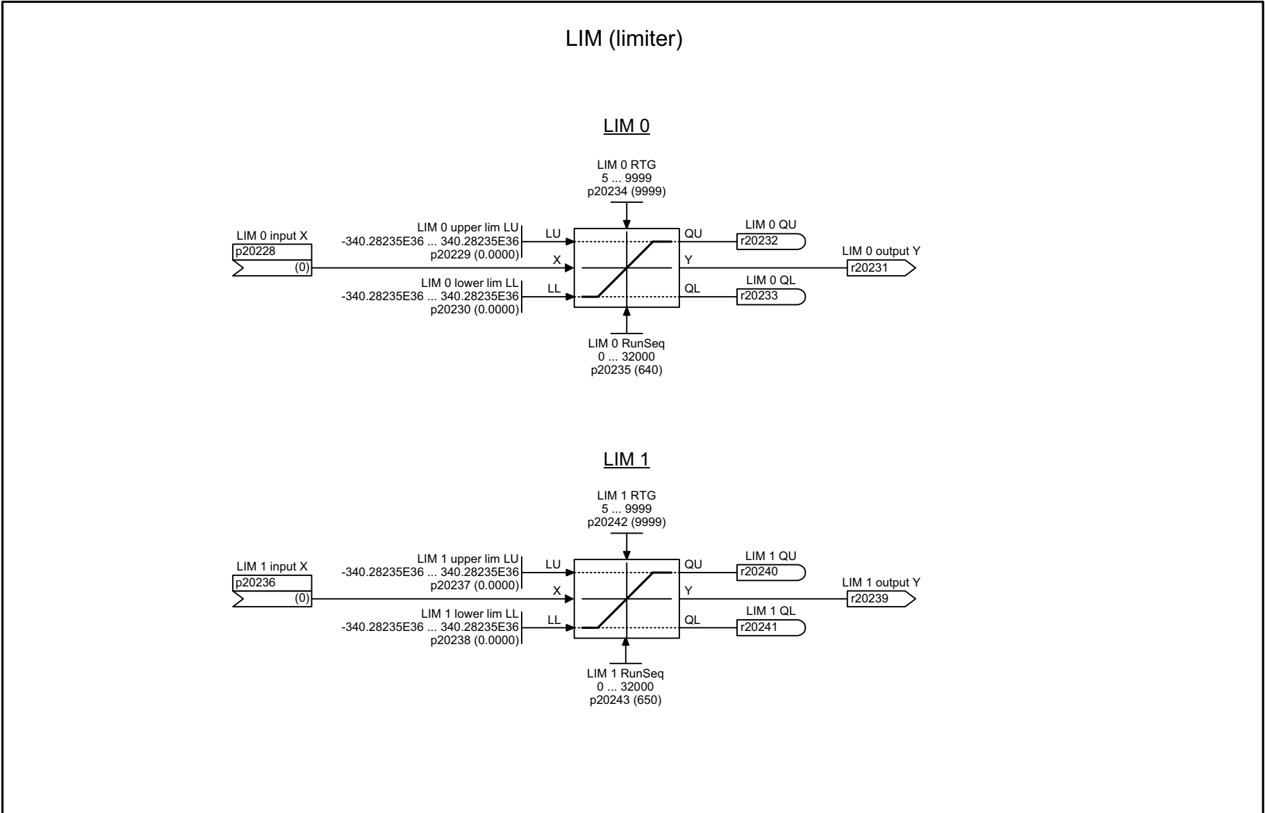
Fig. 3-136 7260 – LIM 0 ... 1
