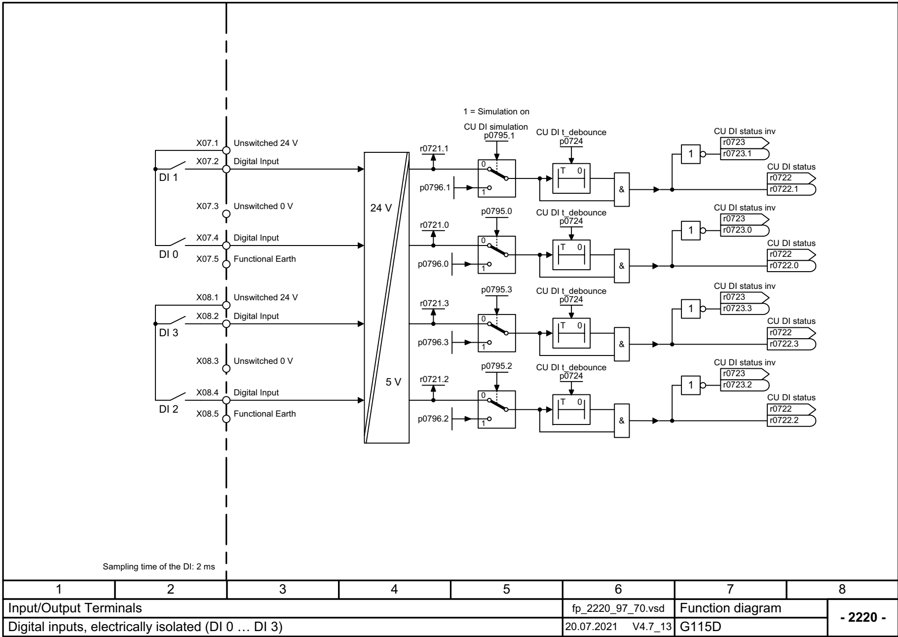
Fig. 3-6 2220 – Digital inputs, electrically isolated (DI 0 ... DI 3)
