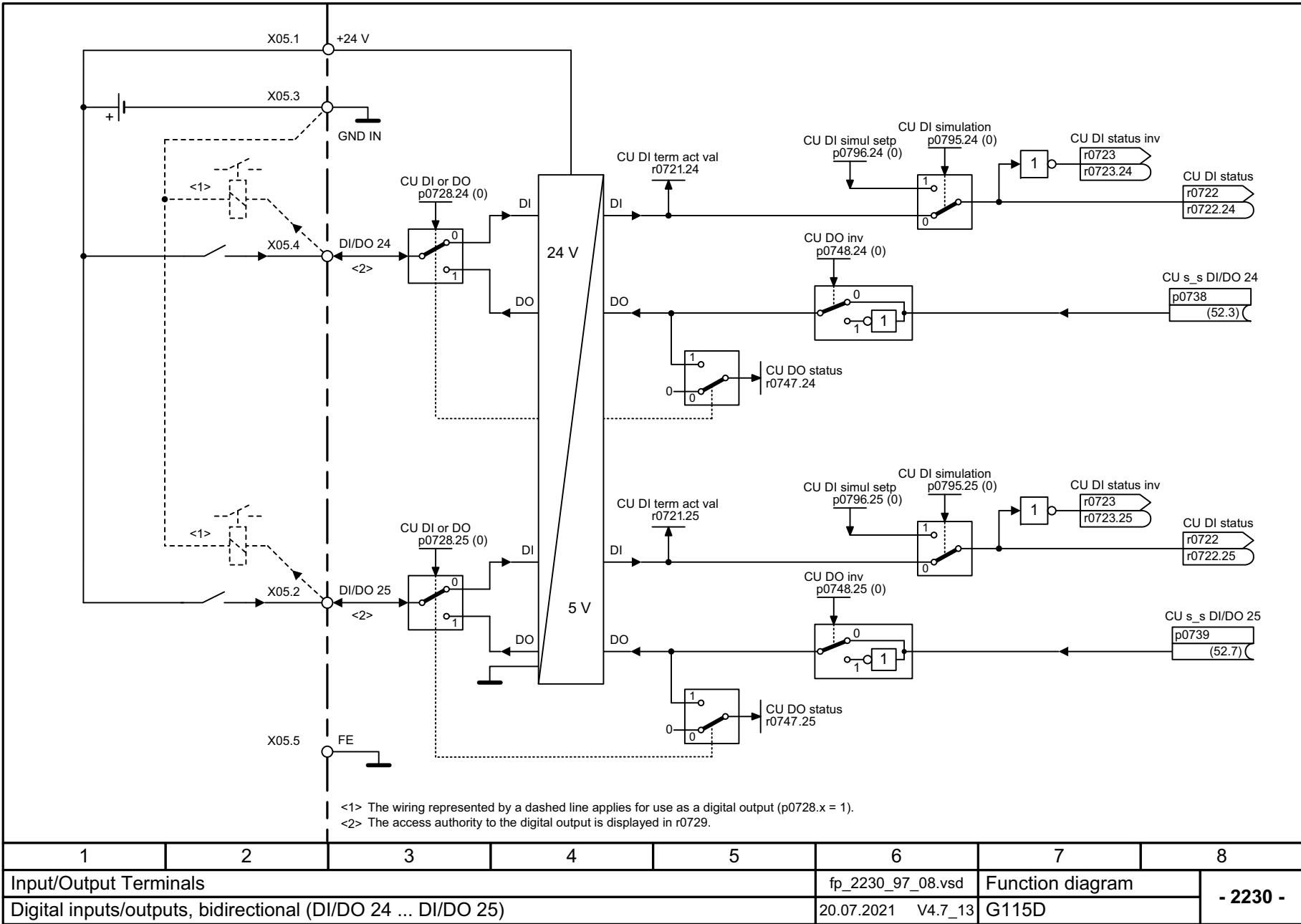
Fig. 3-7 2230 – Digital inputs/outputs bidirectional (DI/DO 24 ... DI/DO 25)
