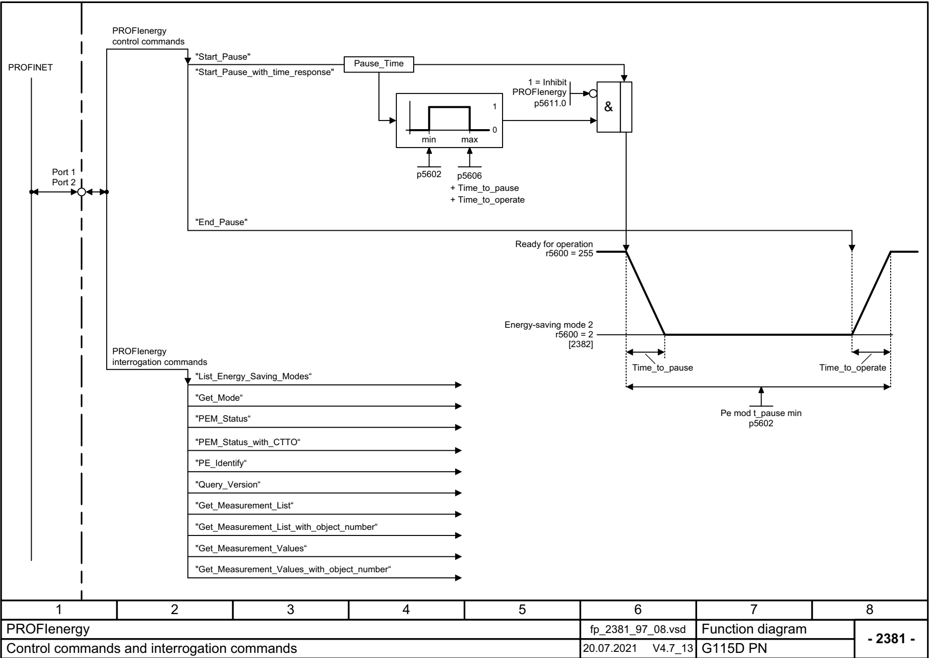
Fig. 3-12 2381 – Control commands and interrogation commands
