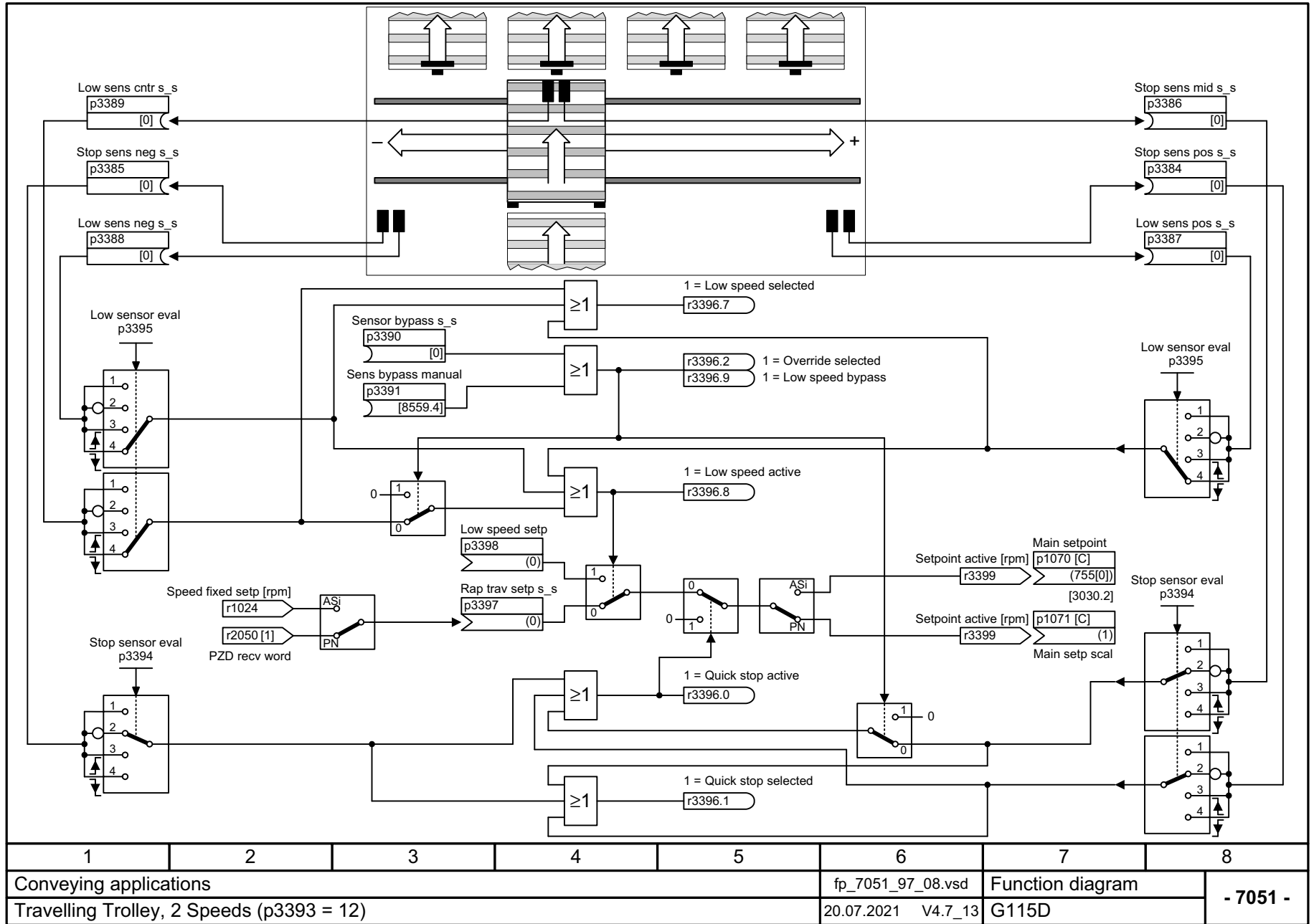
Fig. 3-119 7051 – Travelling Trolley, 2 Speeds (p3393 = 12)
