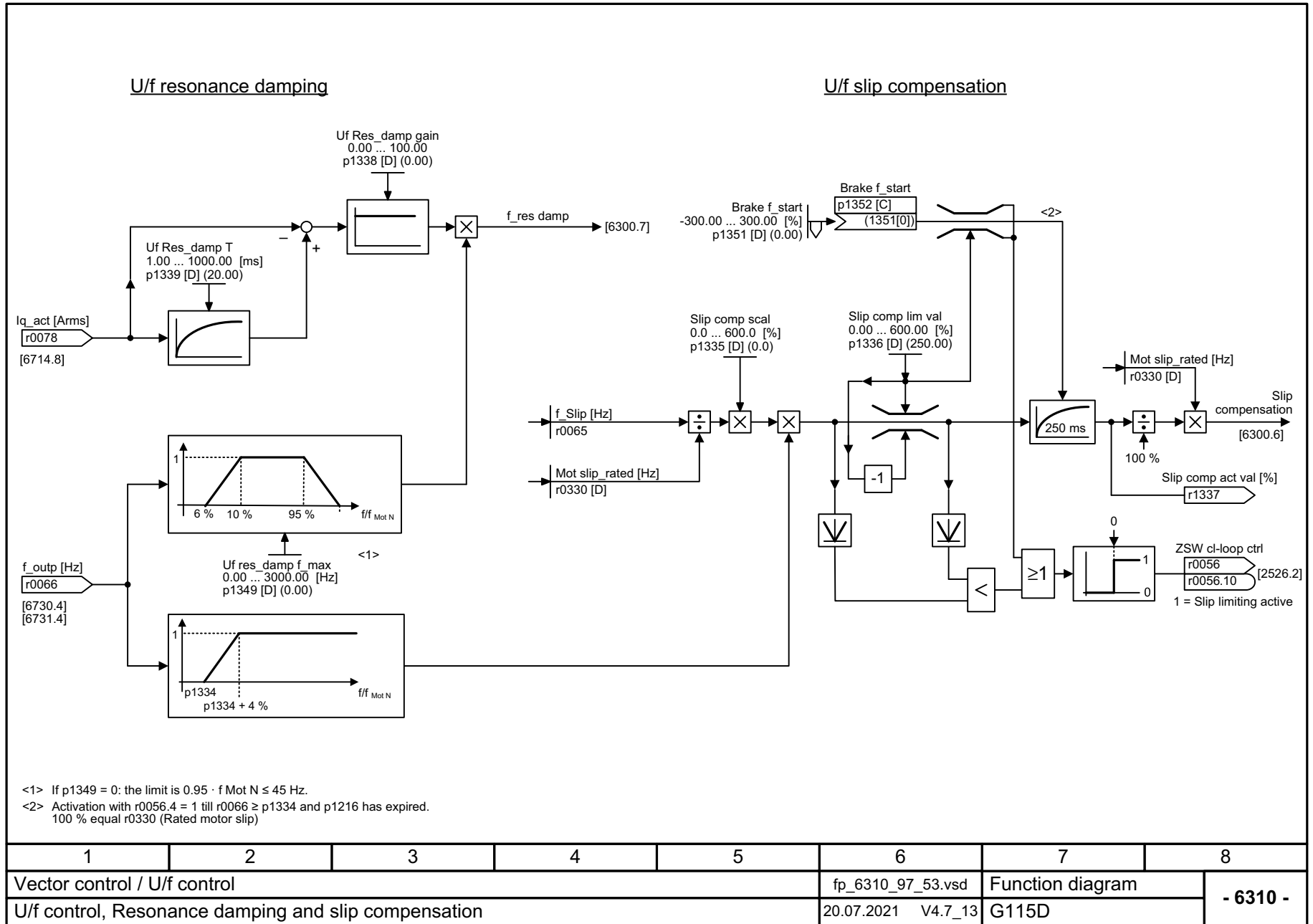
Fig. 3-87 6310 – U/f control, resonance damping and slip compensation
