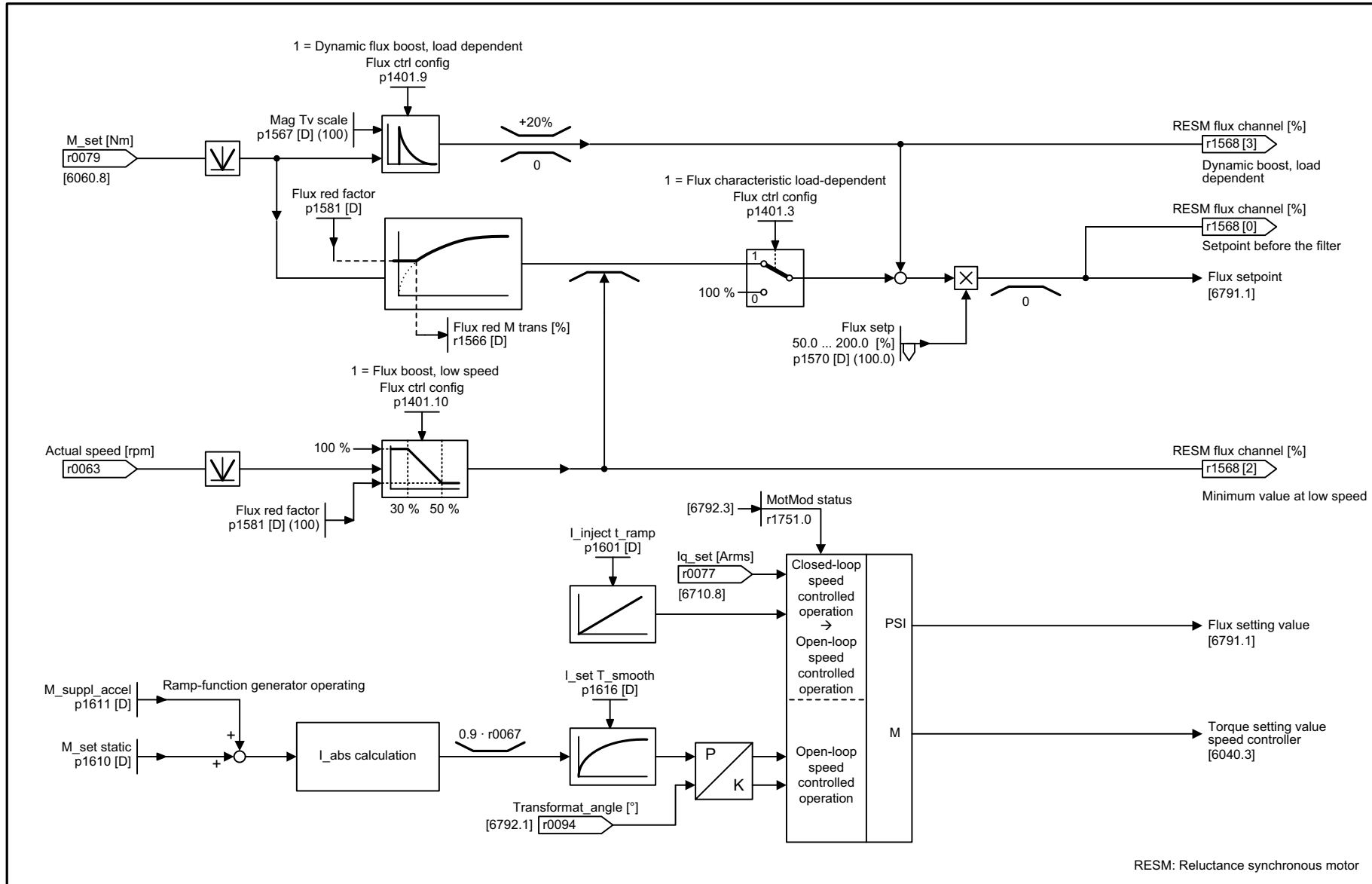
Fig. 3-102 6790 – Flux setpoint (RESM, p0300 = 6xx)
