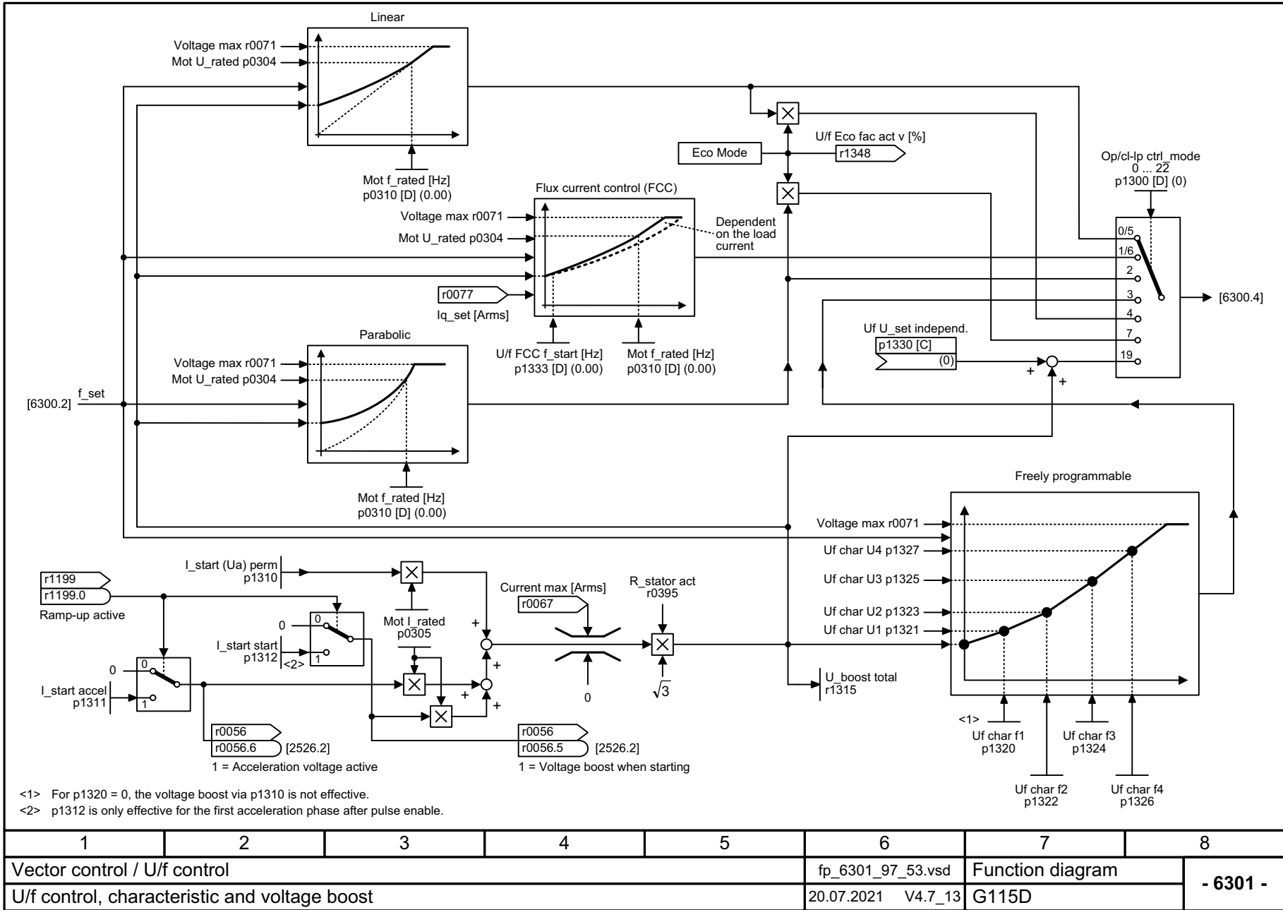
Fig. 3-86 6301 – U/f control, characteristic and voltage boost
