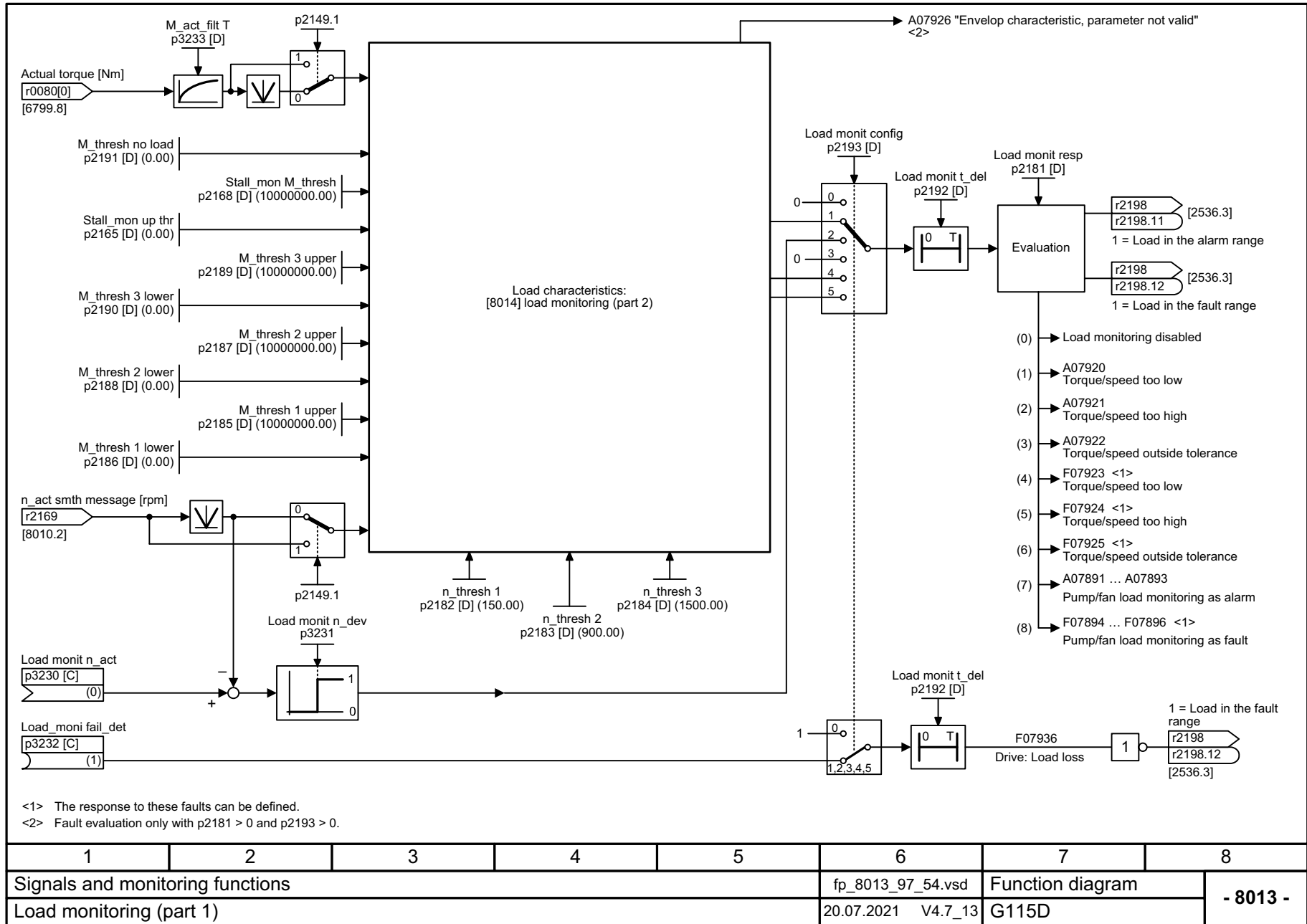
Fig. 3-148 8013 – Load monitoring (Part 1)
