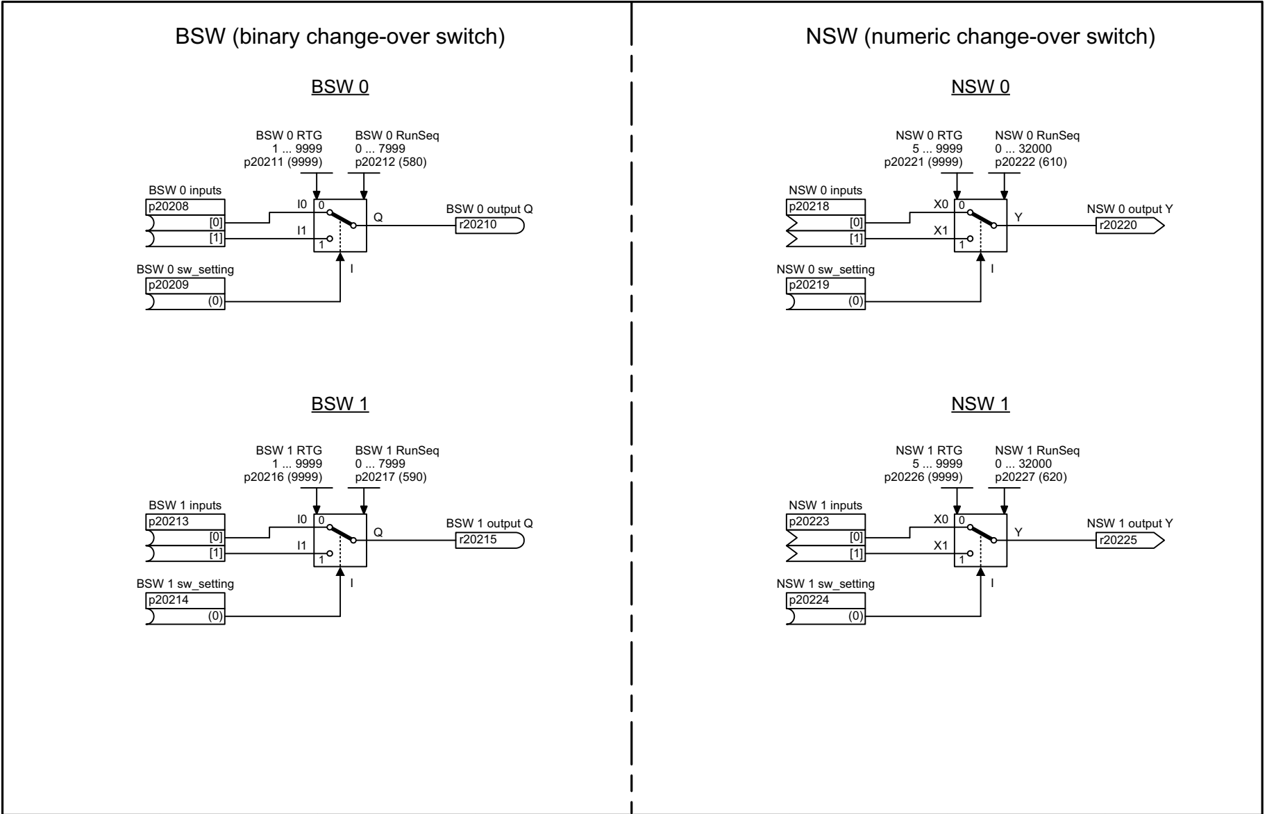
Fig. 3-135 7250 – BSW 0 ... 1, NSW 0 ... 1
