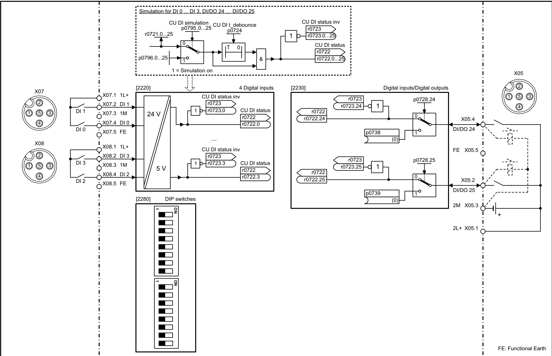
Fig. 3-5 2201 – Connection overview
