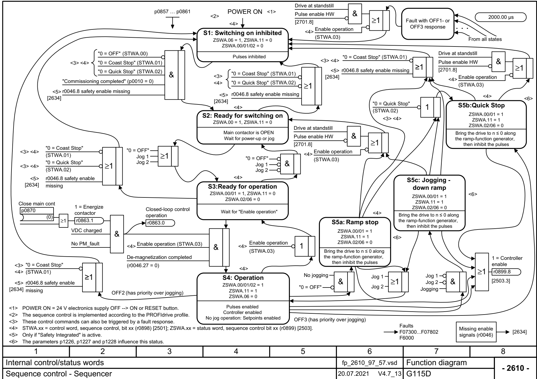
Fig. 3-56 2610 – Sequence control - Sequencer
