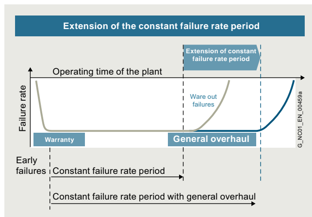
Extension of phases with a constant failure rate
