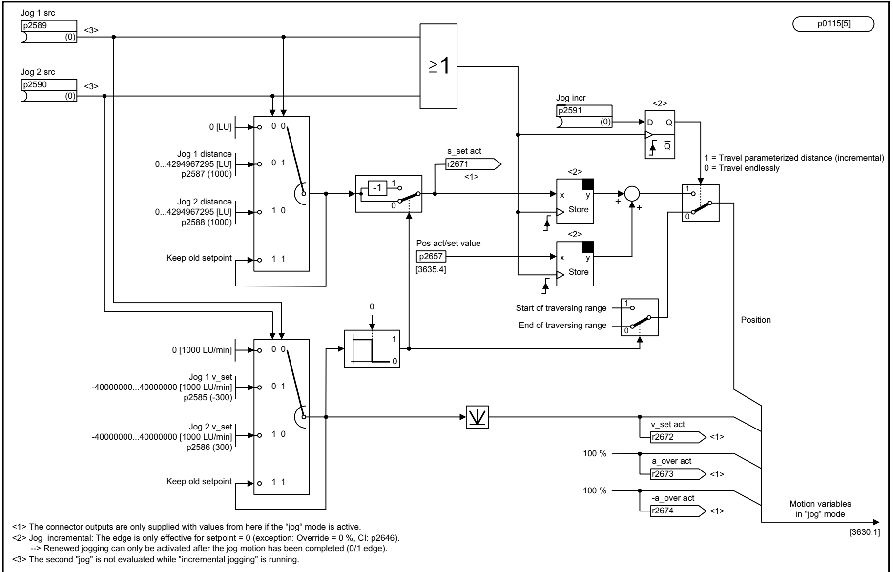
Fig. 3-157 36110 – Jog mode (r0108.4 = 1)
