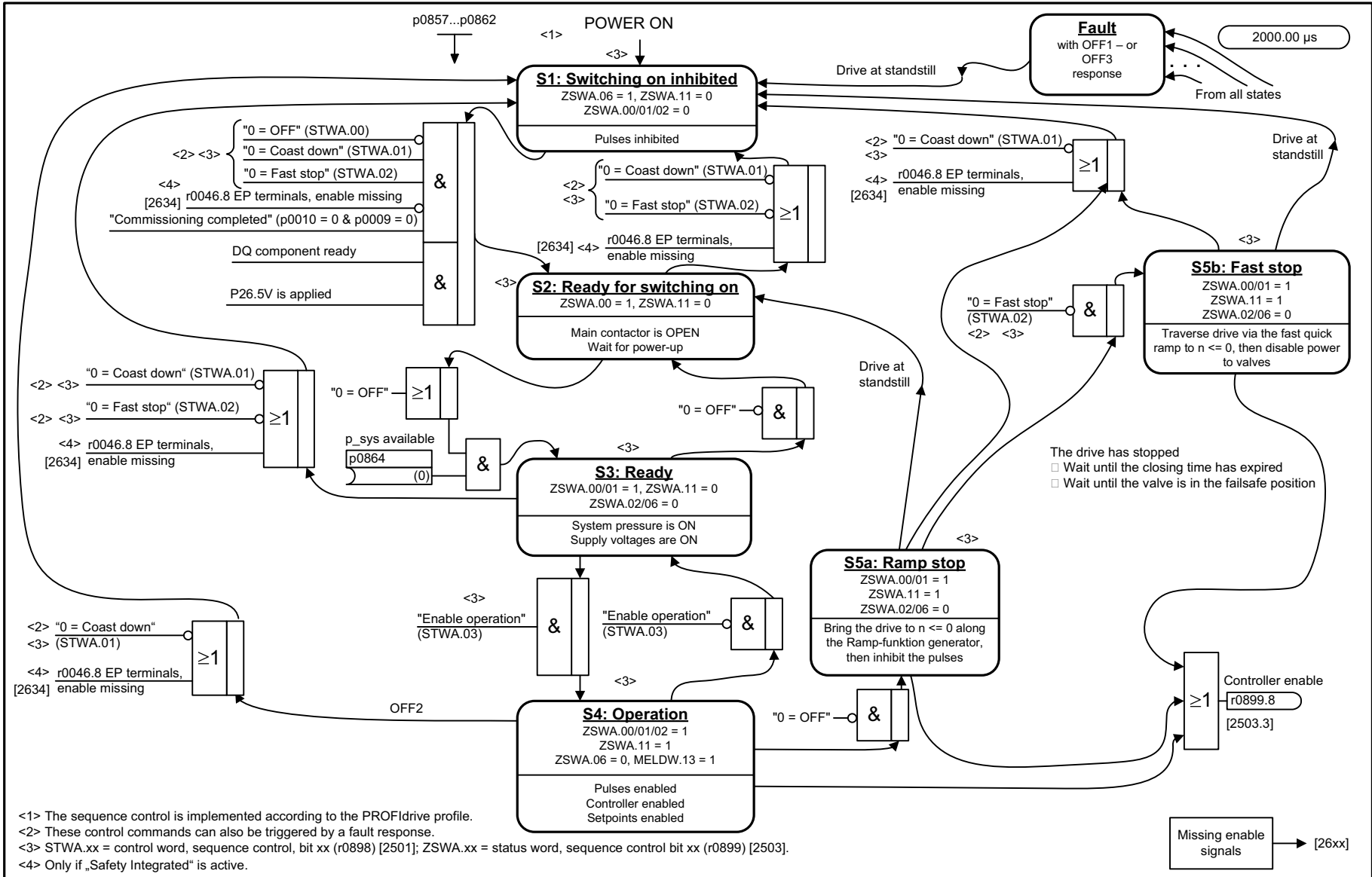
Fig. 3-193 4985 – Sequencer
