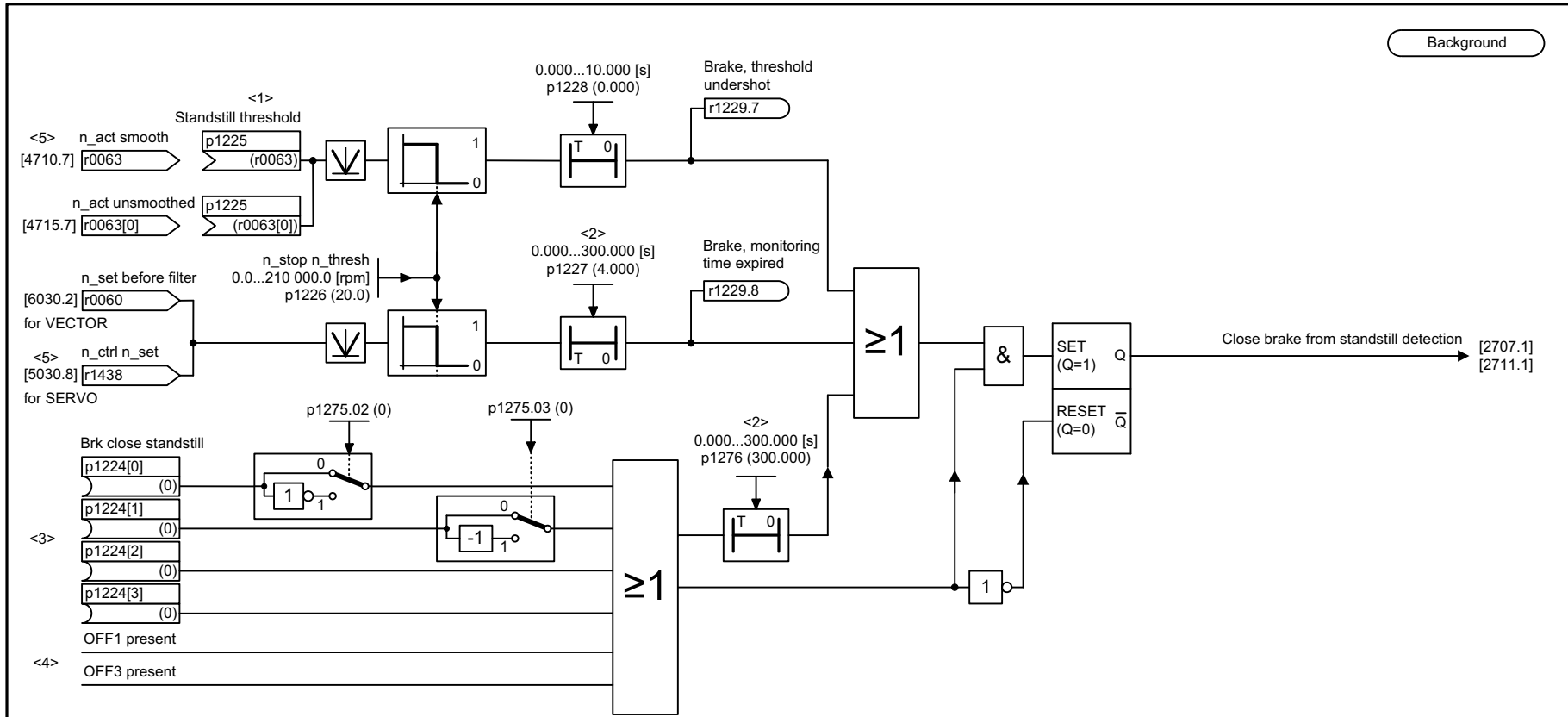
Fig. 3-106 2704 – Extended brake control, zero-speed detection (r0108.14 = 1)
