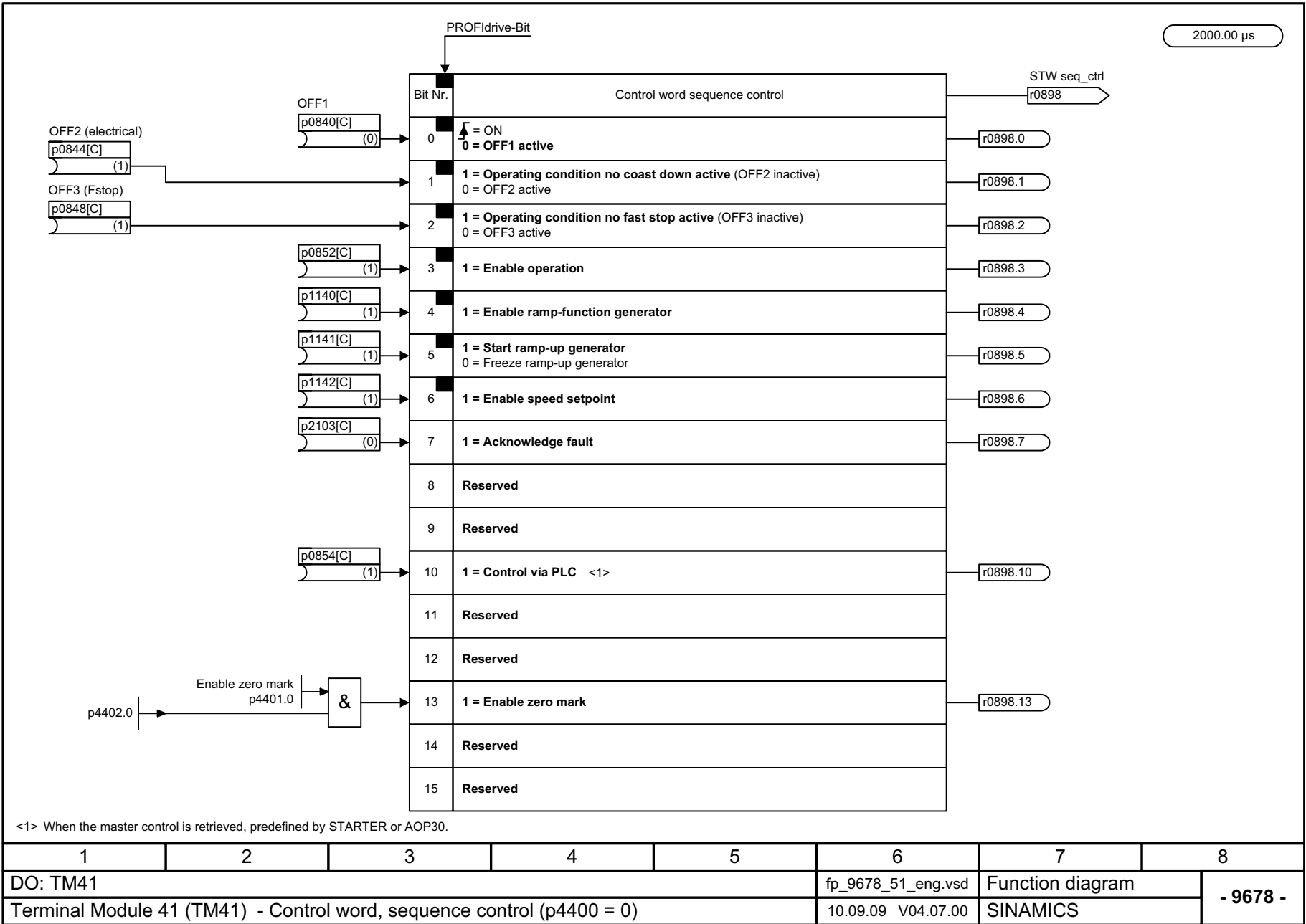
Fig. 3-370 9678 – Control word, sequence control (p4400 = 0)
