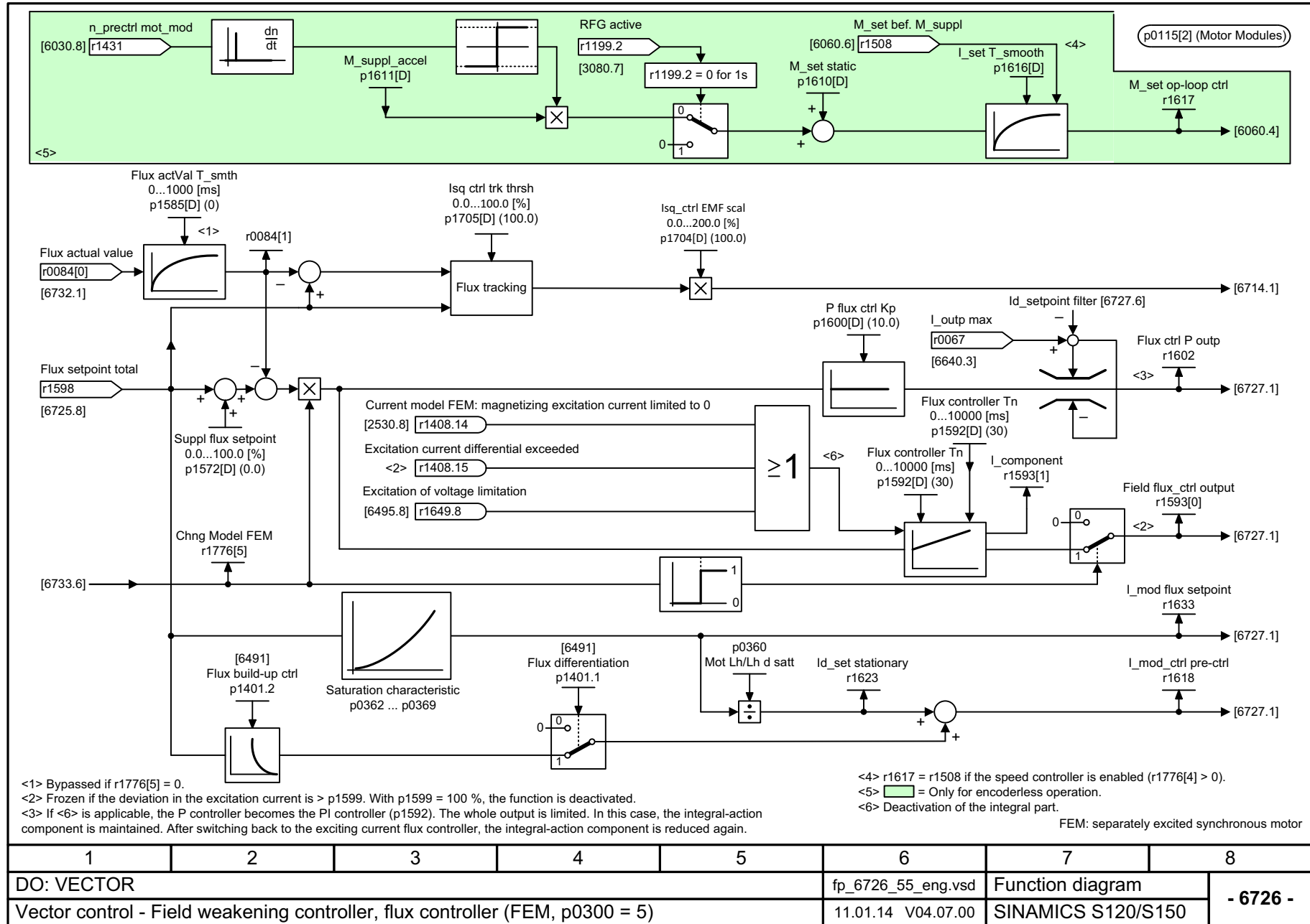
Fig. 3-244 6726 – Field weakening controller, flux controller (FEM, p0300 = 5)
