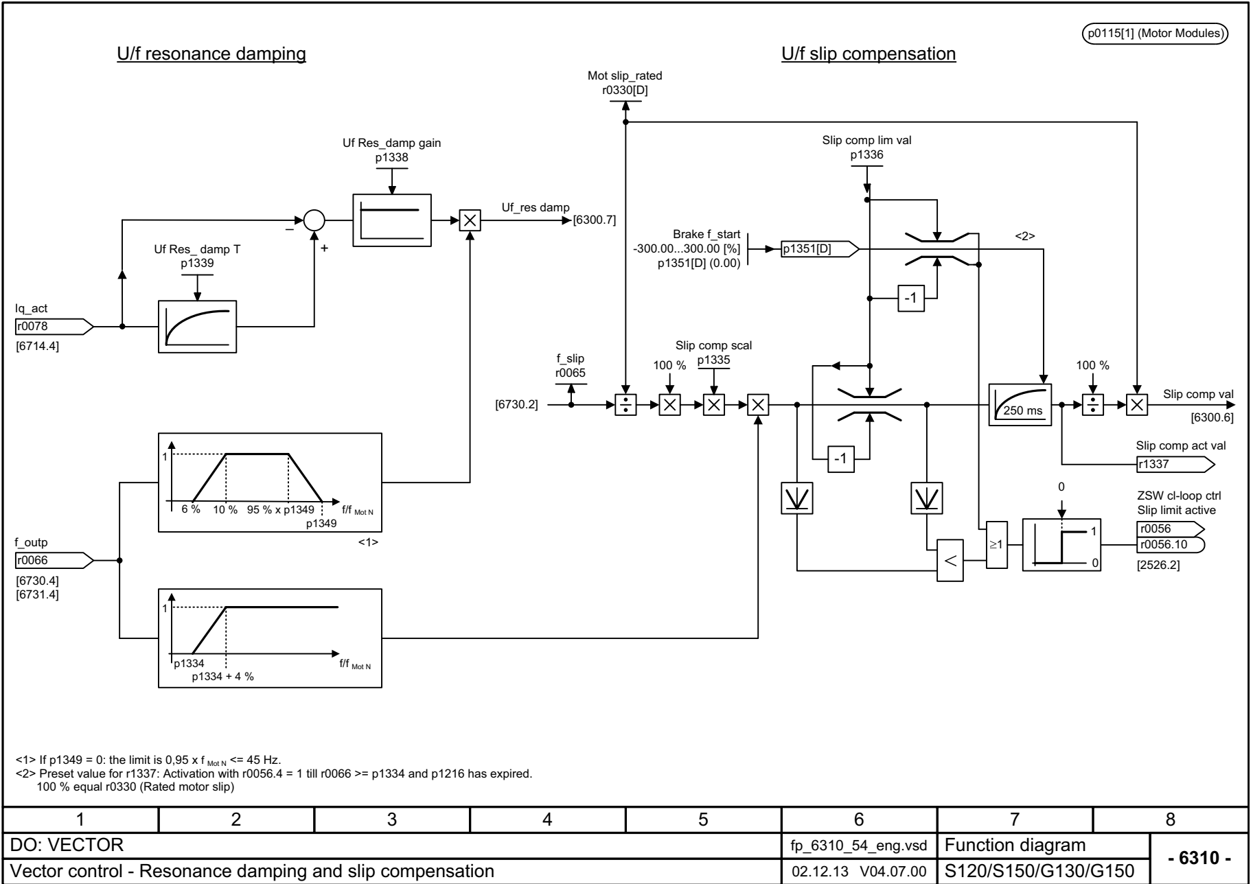
Fig. 3-229 6310 – Resonance damping and slip compensation
