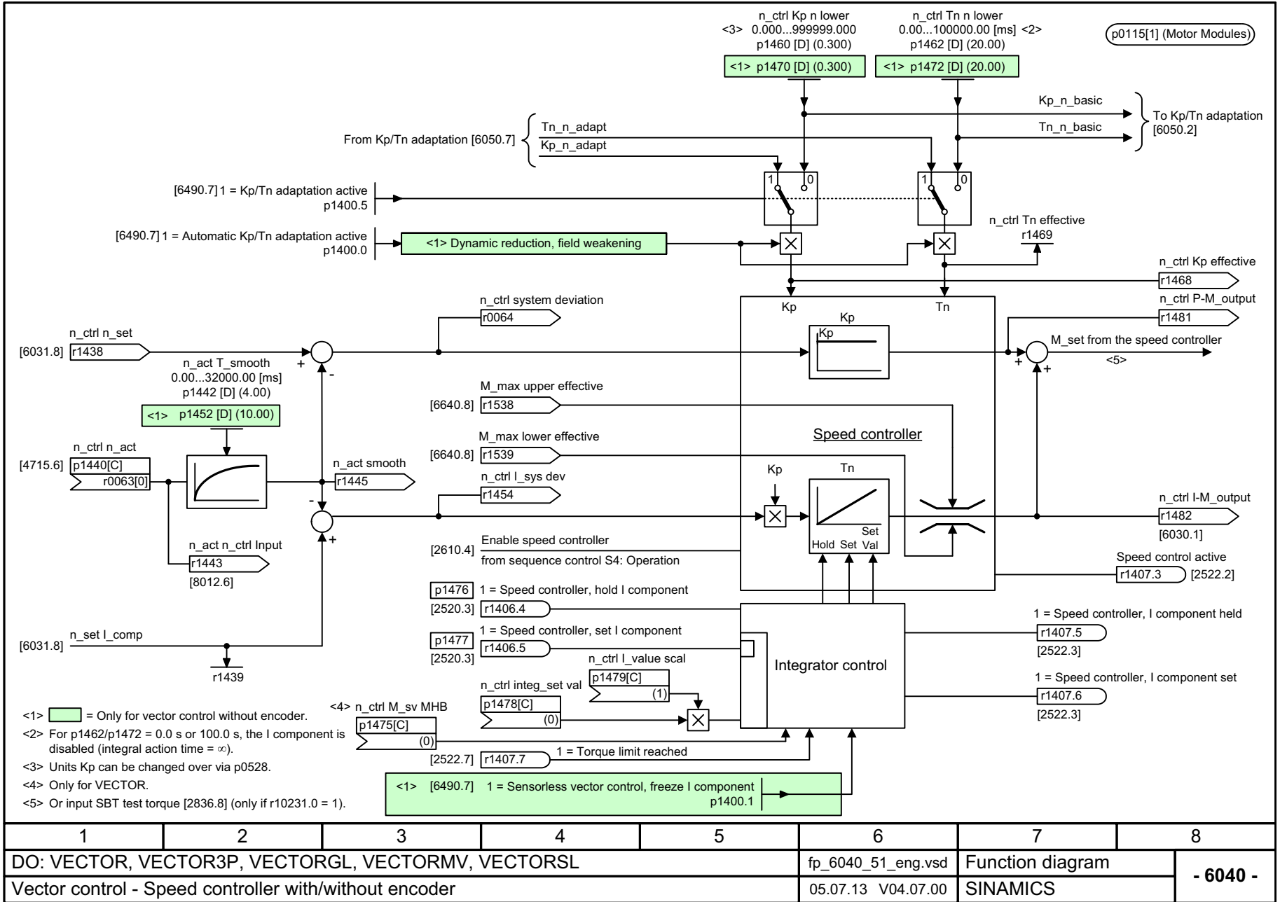
Fig. 3-223 6040 – Speed controller with/without encoder
