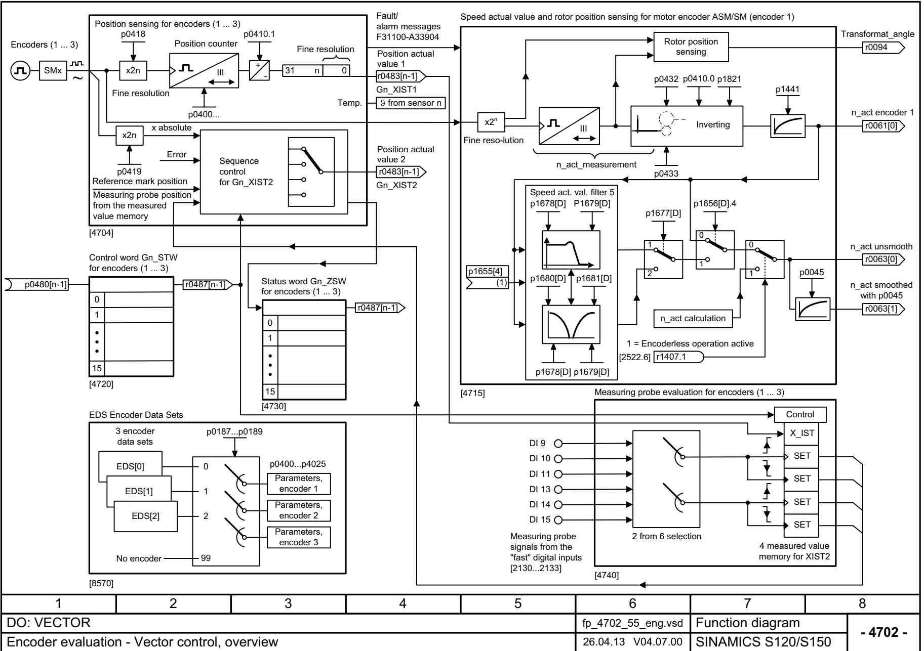
Fig. 3-177 4702 – Vector control, overview
