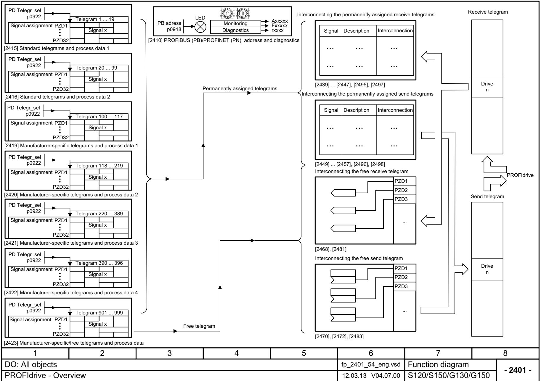
Fig. 3-32 2401 – Overview
