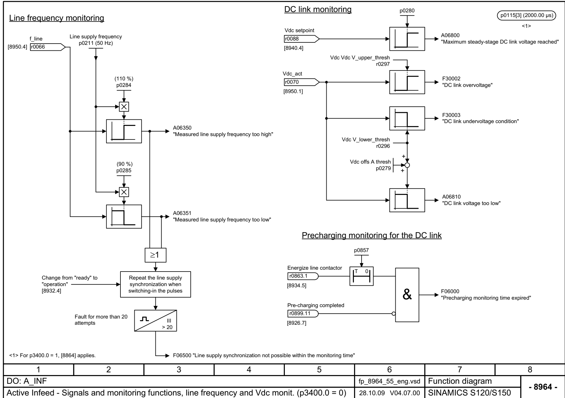
Fig. 3-329 8964 – Signals and monitoring functions: line frequency/Vdc monit. (p3400.0 = 0)
