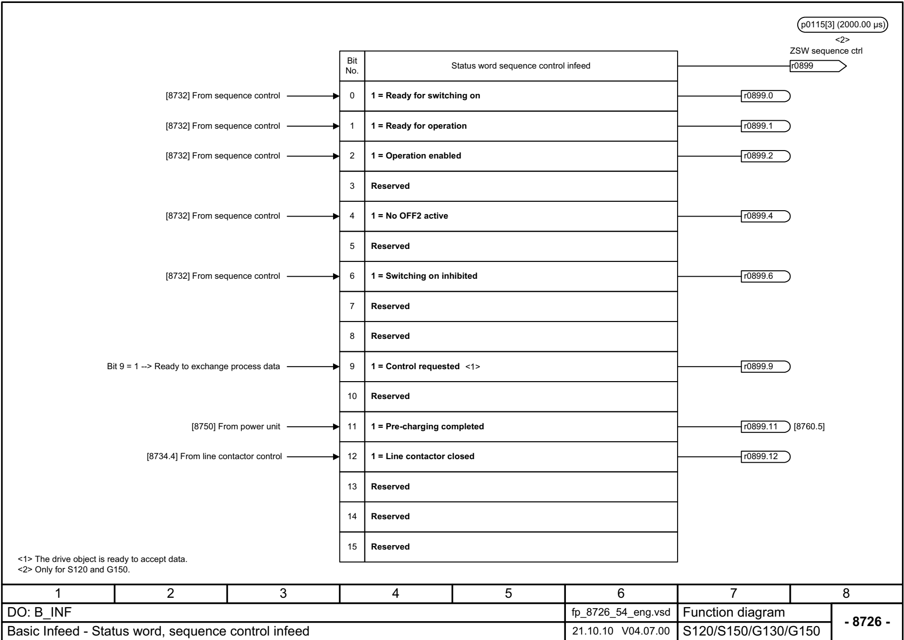
Fig. 3-302 8726 – Status word, sequence control infeed
