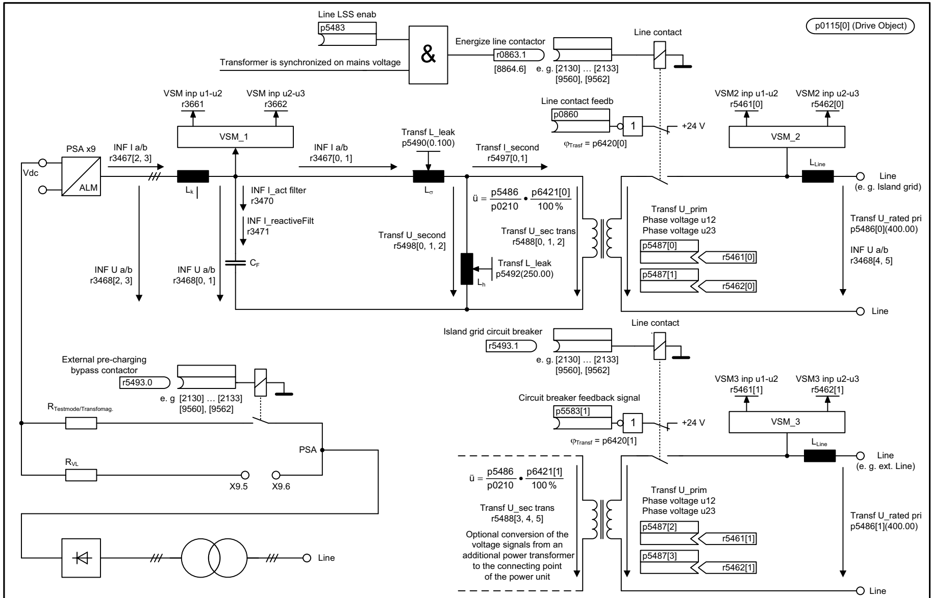
Fig. 3-271 7990 – Transformer model (r0108.4 = 1 and p5480 = 1)
