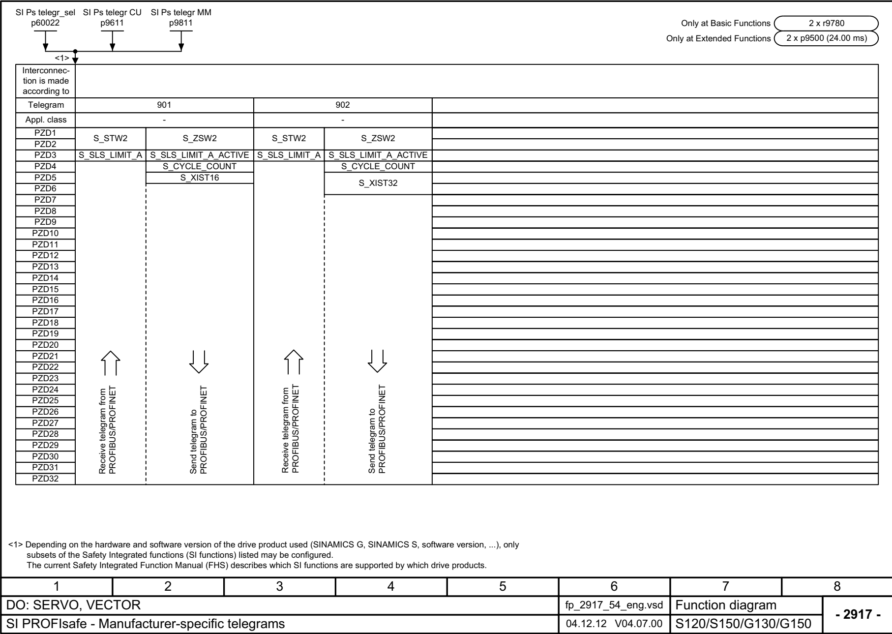
Fig. 3-144 2917 – Manufacturer-specific telegrams
