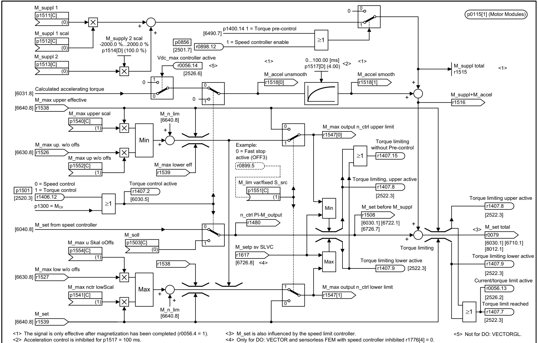
Fig. 3-225 6060 – Torque setpoint
