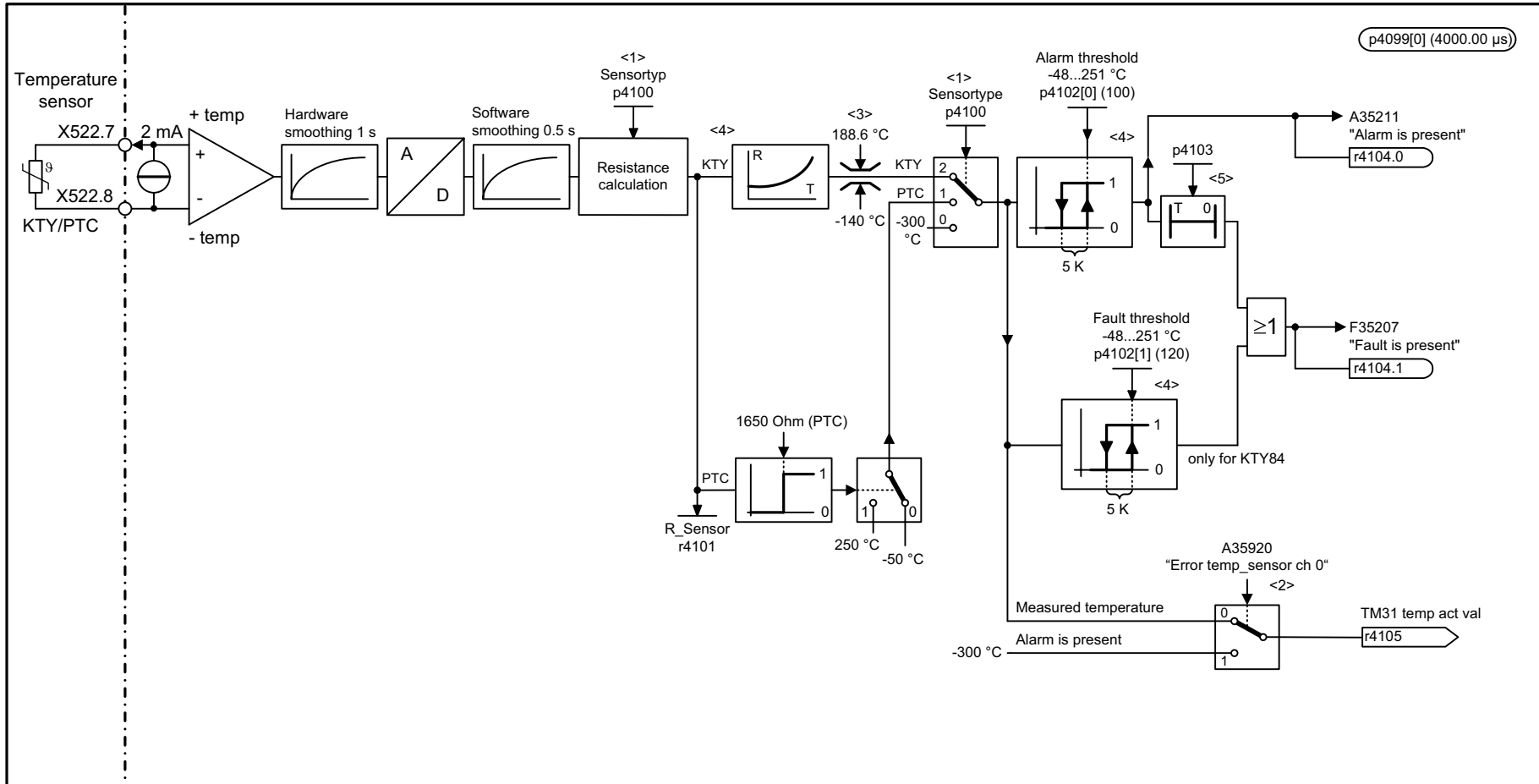
Fig. 3-356 9576 - Temperature evaluation (KTY/PTC)
