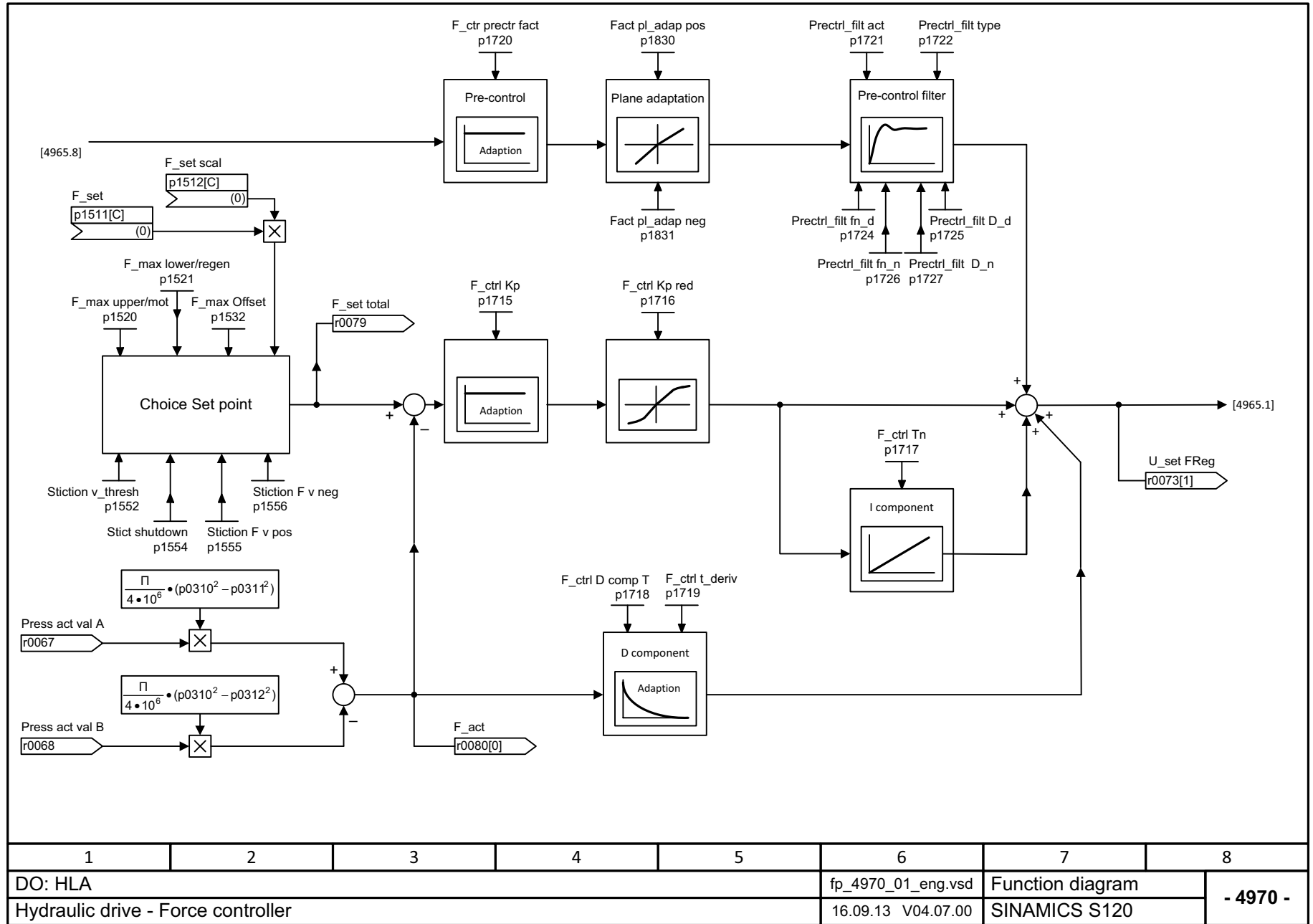
Fig. 3-189 4970 – Force controller
