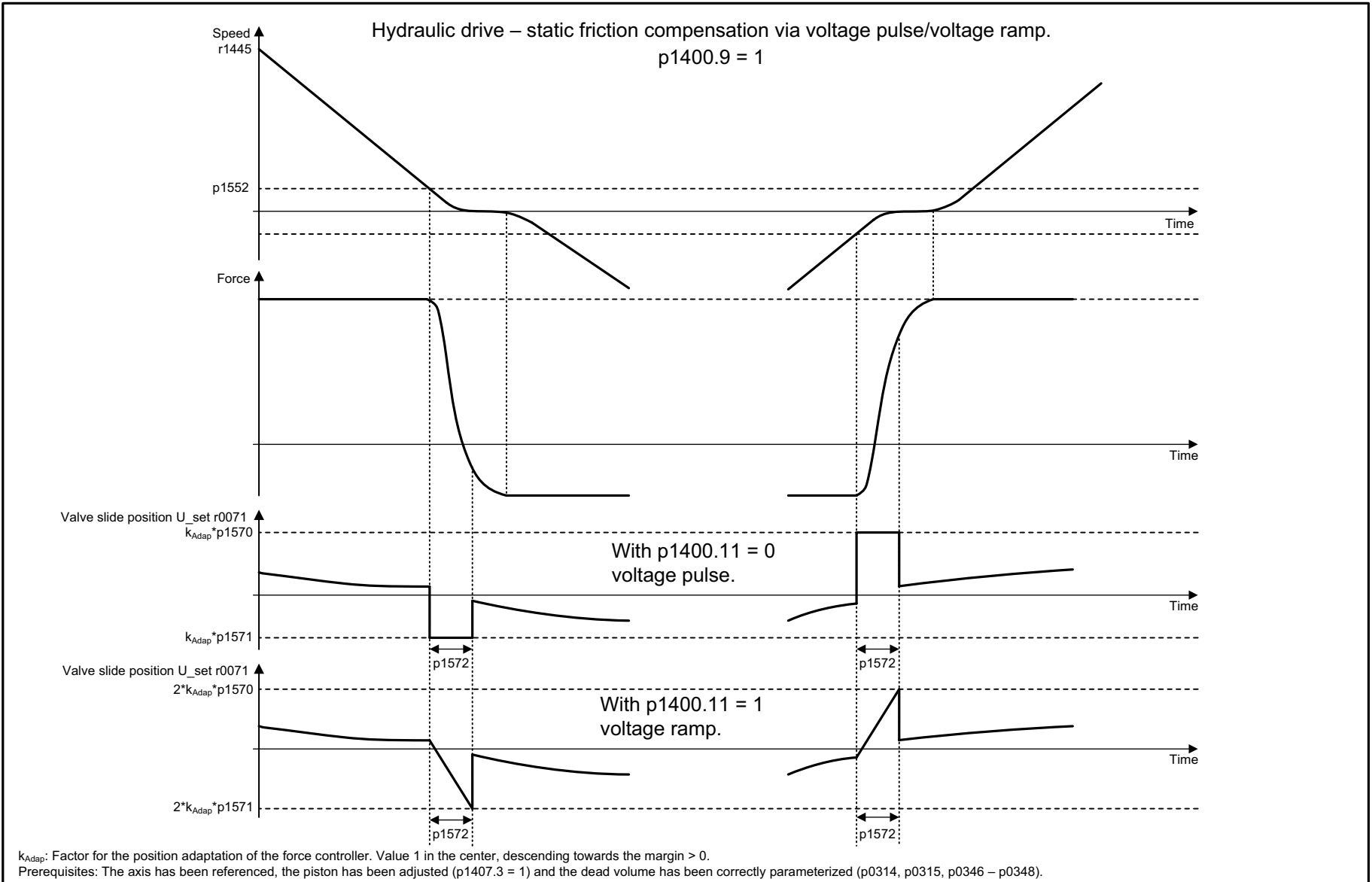
Fig. 3-192 4978 – Static friction compensation via voltage pulse / voltage ramp
