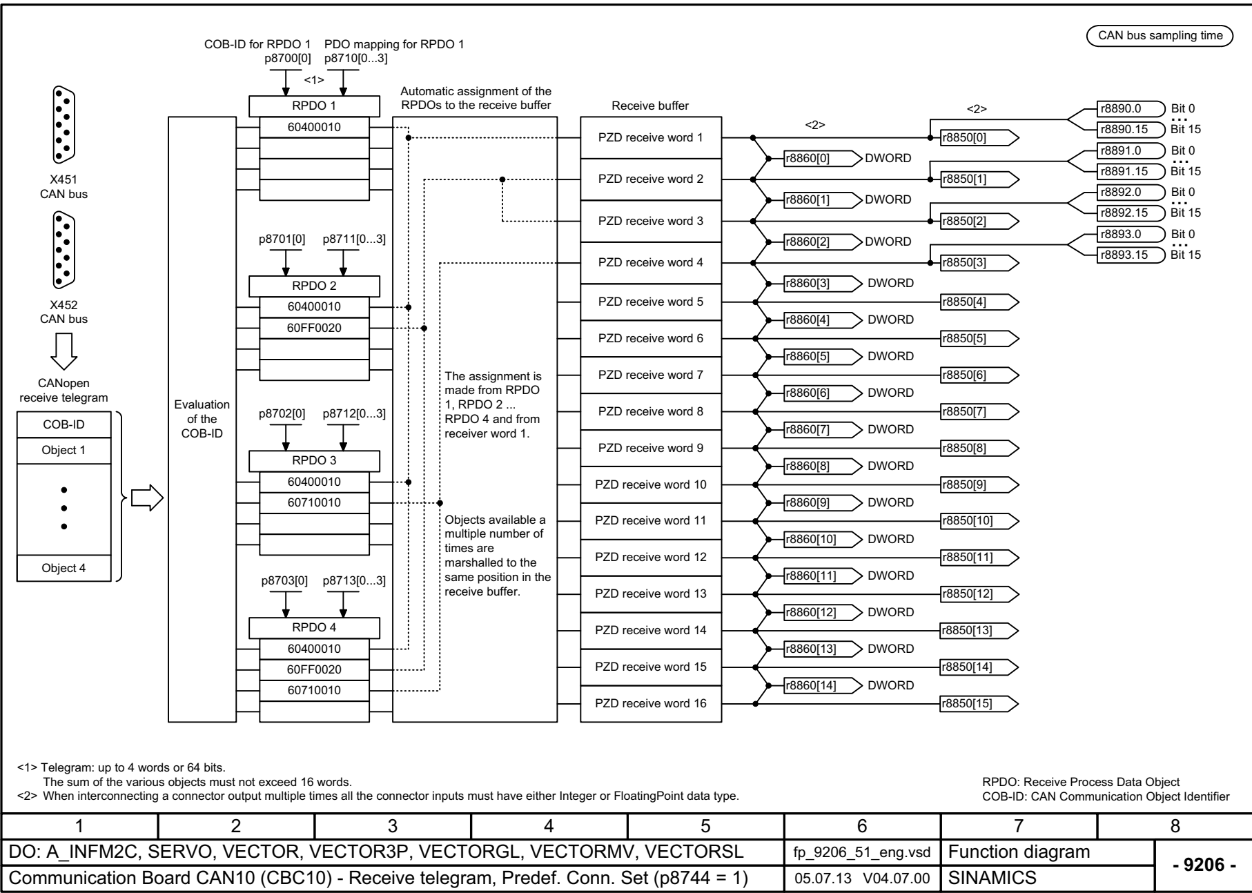
Fig. 3-336 9206 – Receive telegram, Predefined Connection Set (p8744 = 1)
