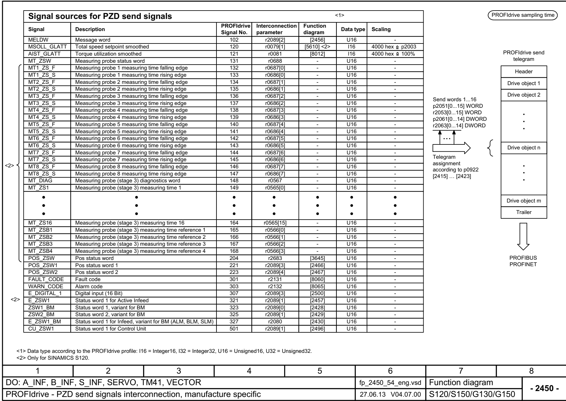
Fig. 3-58 2450 – PZD send signals interconnection, manufacturer-specific
