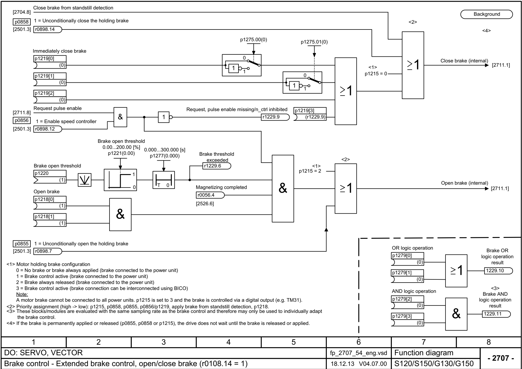
Fig. 3-107 2707 – Extended brake control, open/close brake (r0108.14 = 1)
