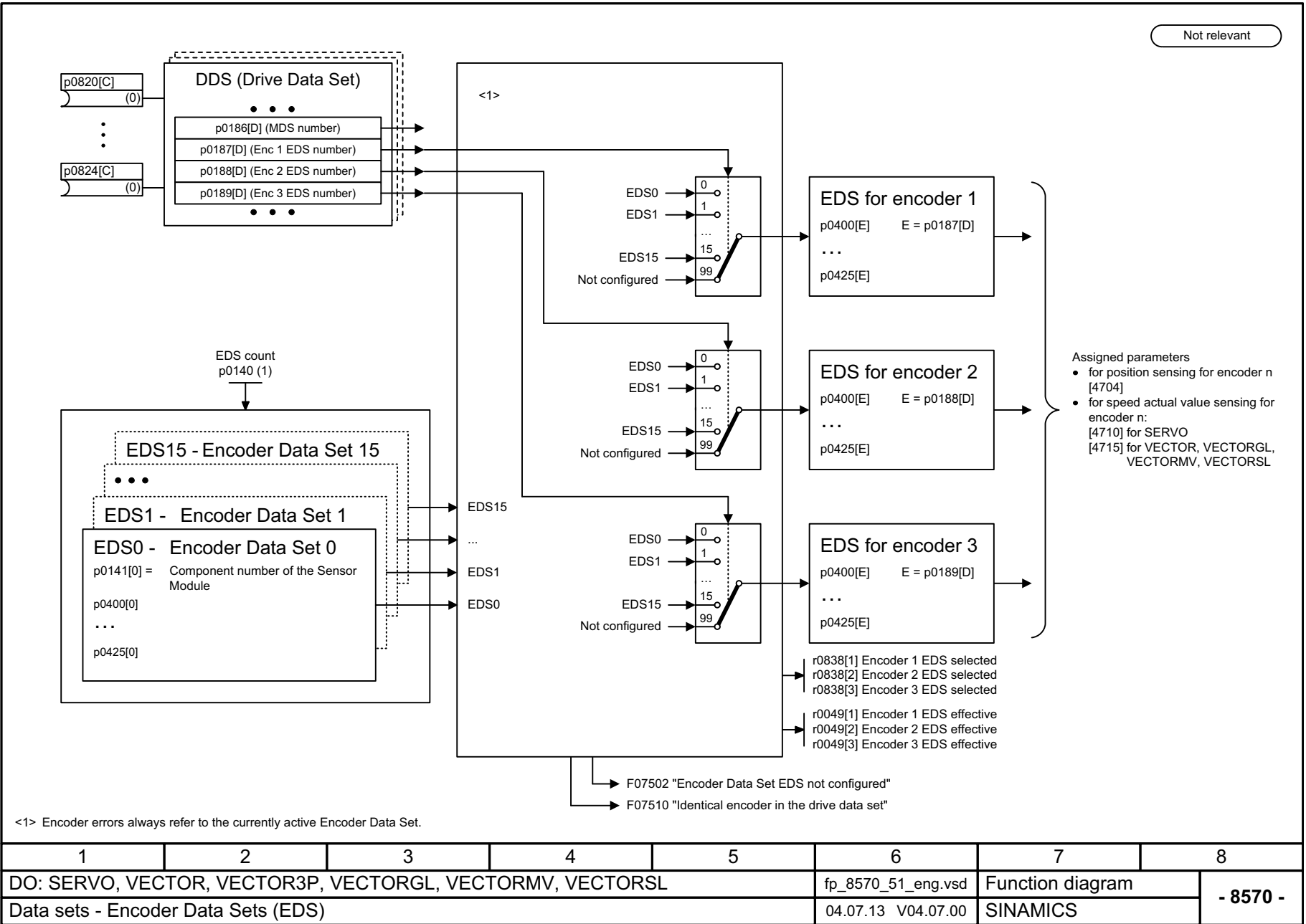
Fig. 3-297 8570 – Encoder Data Sets (EDS)
