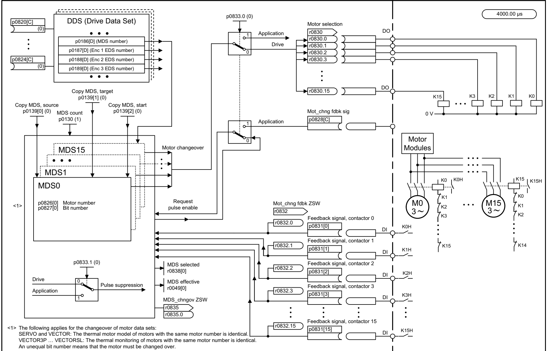
Fig. 3-298 8575 – Motor Data Sets (MDS)
