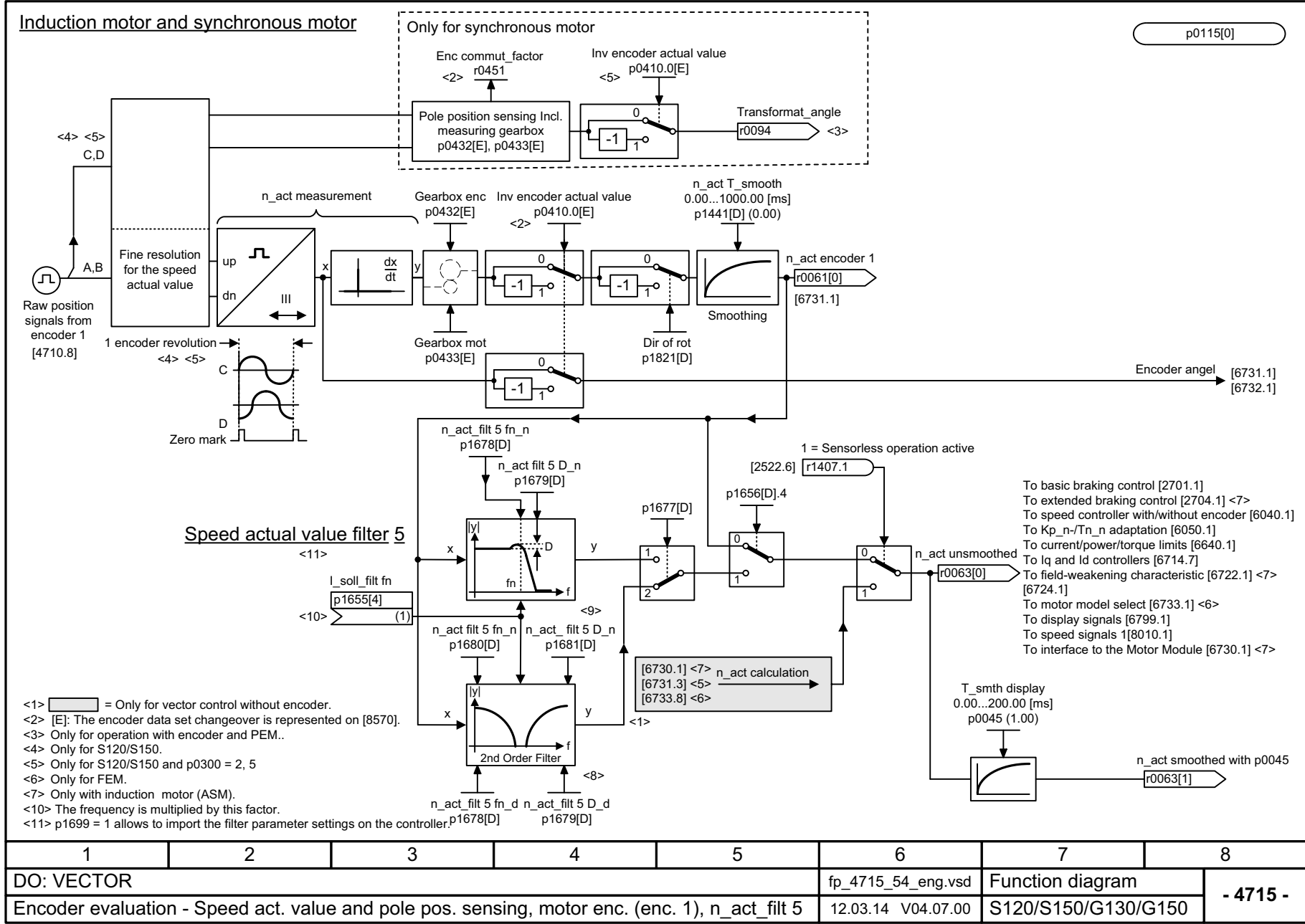
Fig. 3-181 4715 – Speed actual value and pole position sensing, motor encoder (encoder 1), n_act_filt 5
