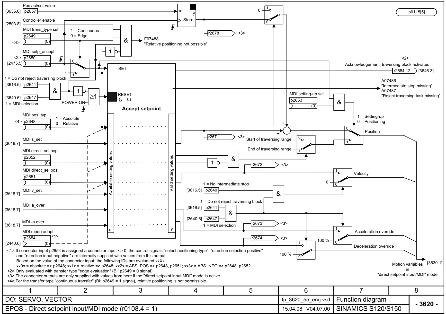
Fig. 3-164 3620 – Direct setpoint input/MDI mode (r0108.4 = 1)
