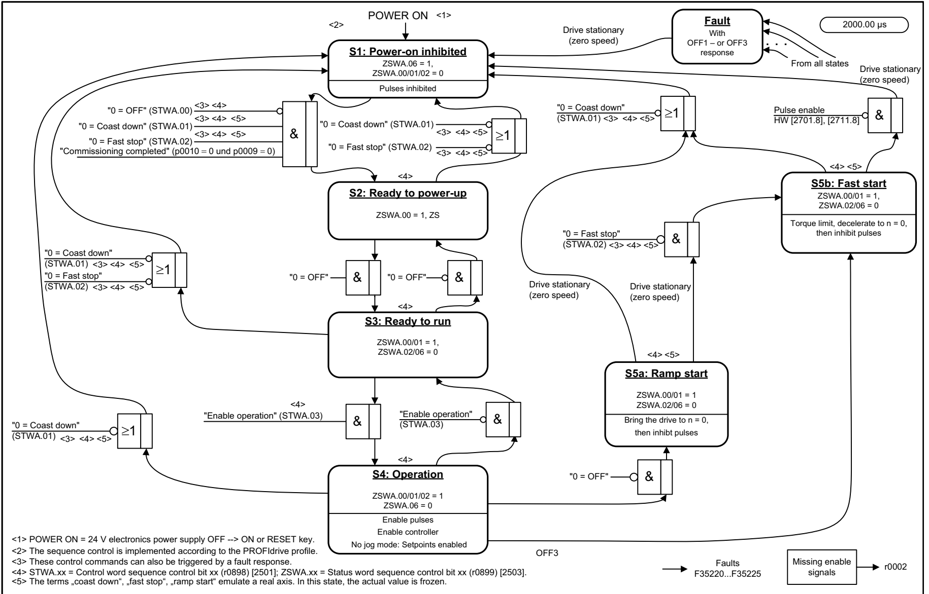
Fig. 3-374 9682 – Sequencer (p4400 = 0)
