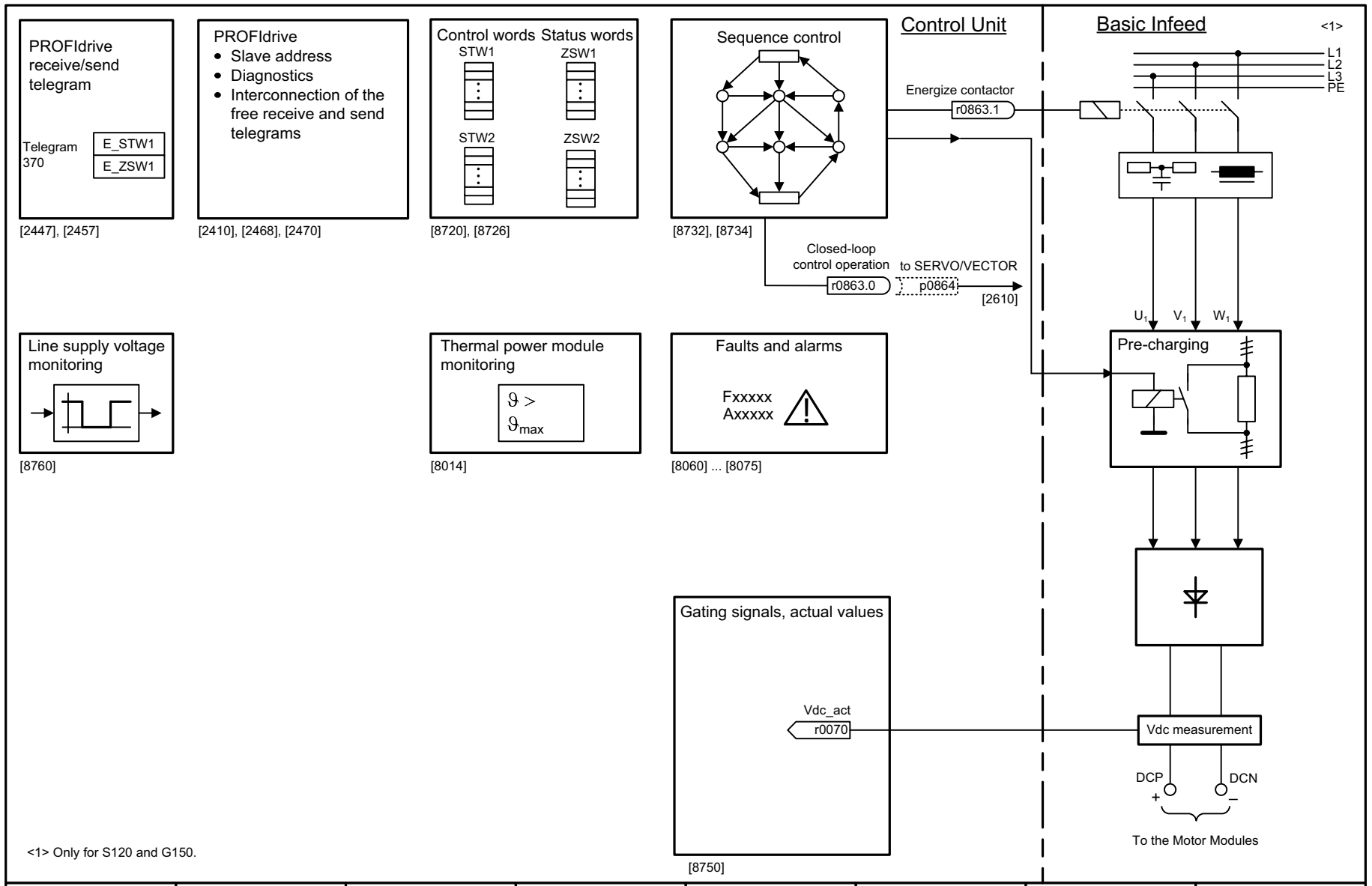
Fig. 3-300 8710 – Overview
