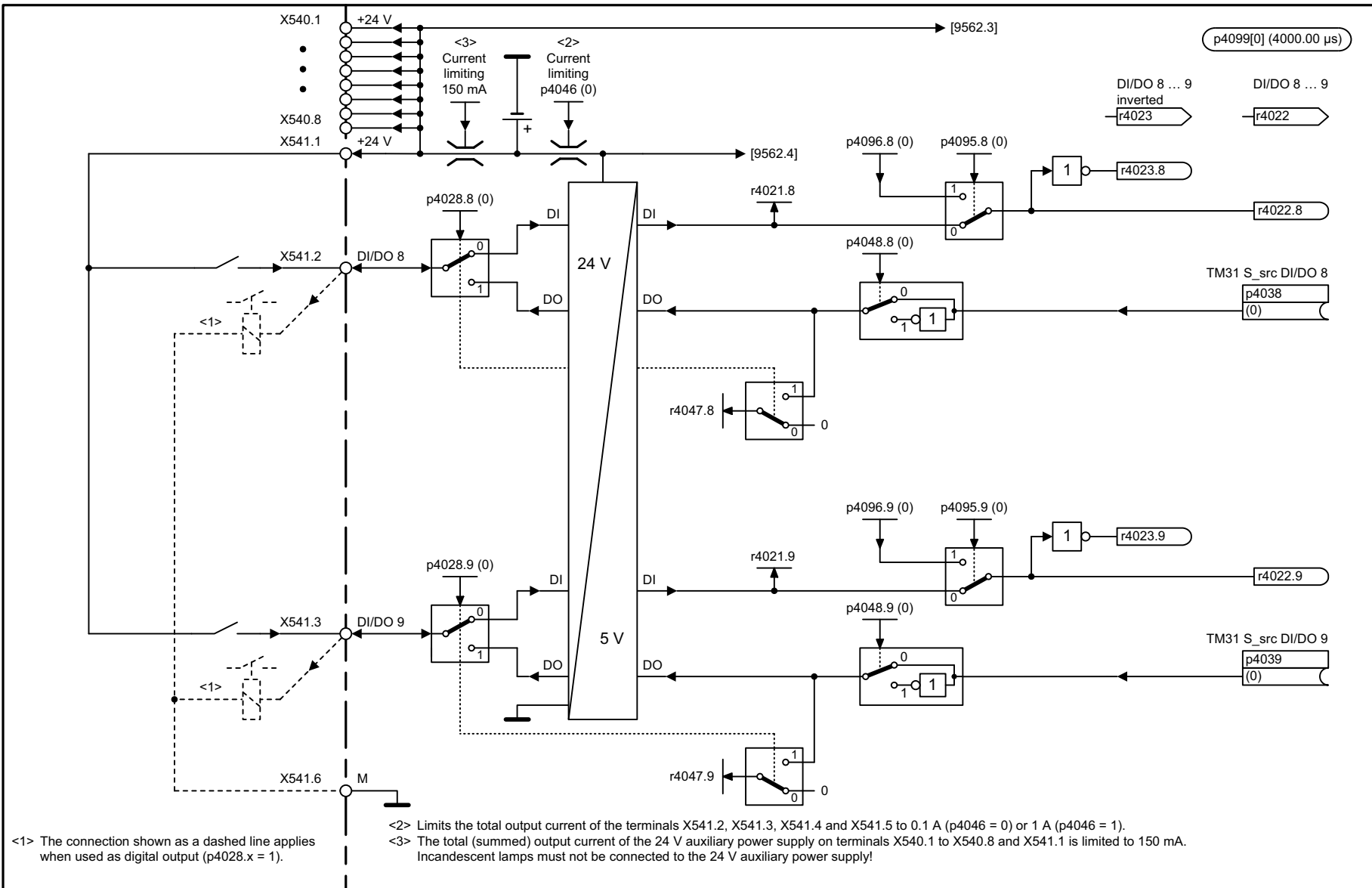
Fig. 3-351 9560 – Digital inputs/outputs, bidirectional (DI/DO 8 ... DI/DO 9)
