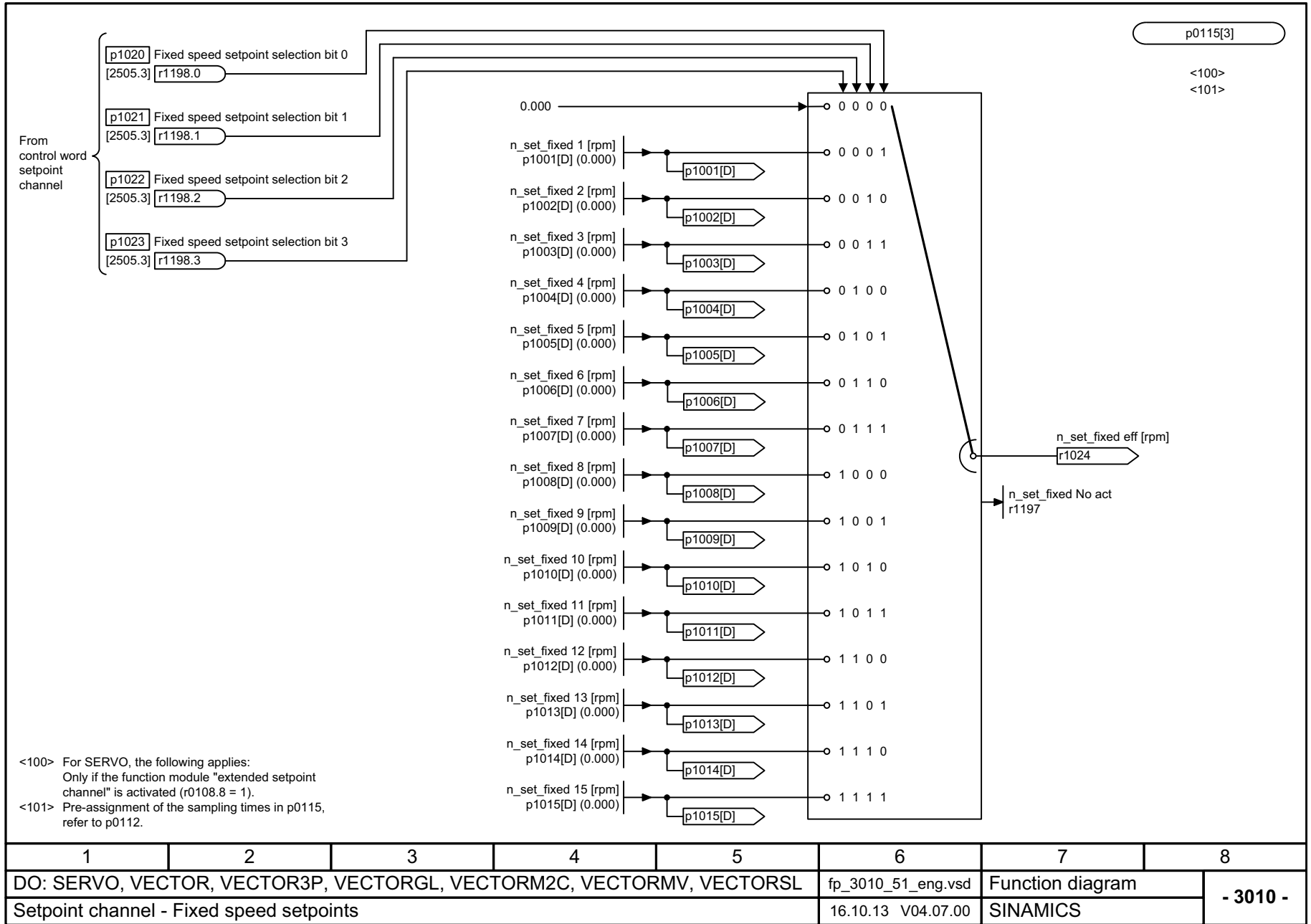
Fig. 3-146 3010 – Fixed speed setpoints
