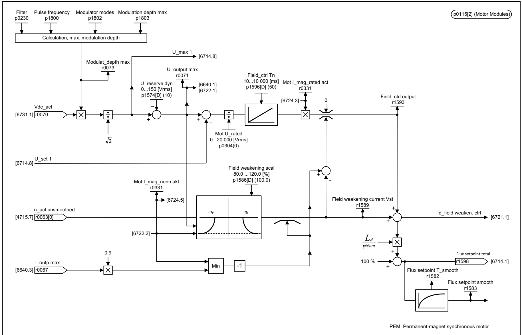
Fig. 3-242 6724 – Field weakening controller (PEM, p0300 = 2)
