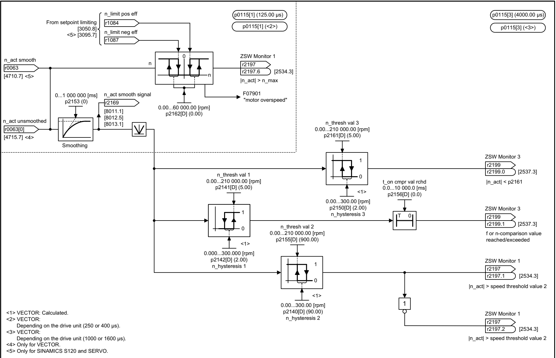
Fig. 3-281 8010 – Speed signals 1
