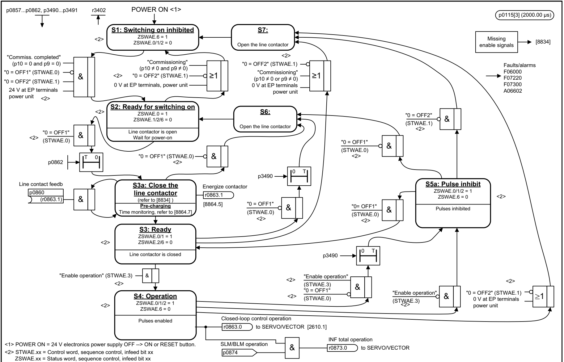
Fig. 3-311 8832 - Sequencer
