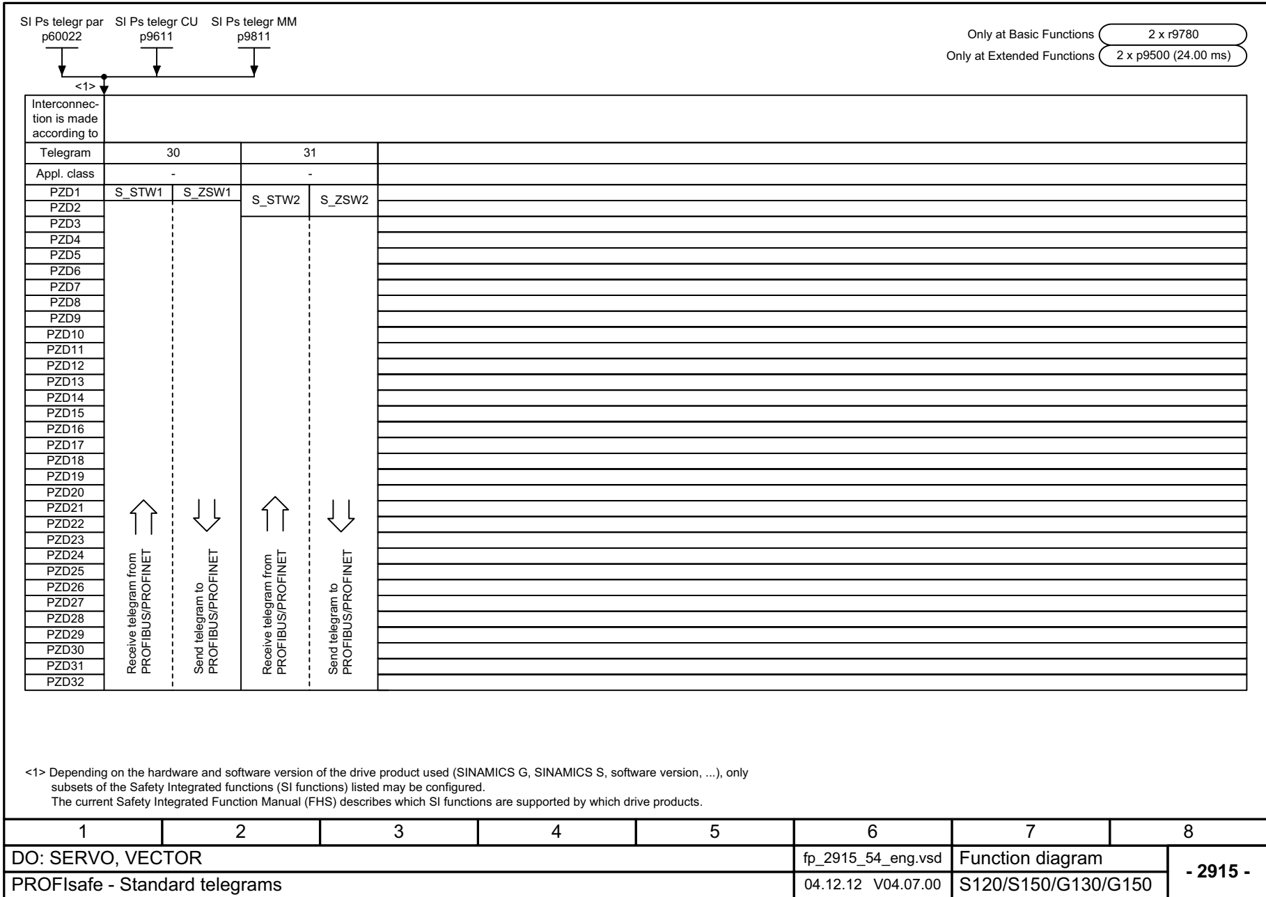
Fig. 3-143 2915 – Standard telegrams
