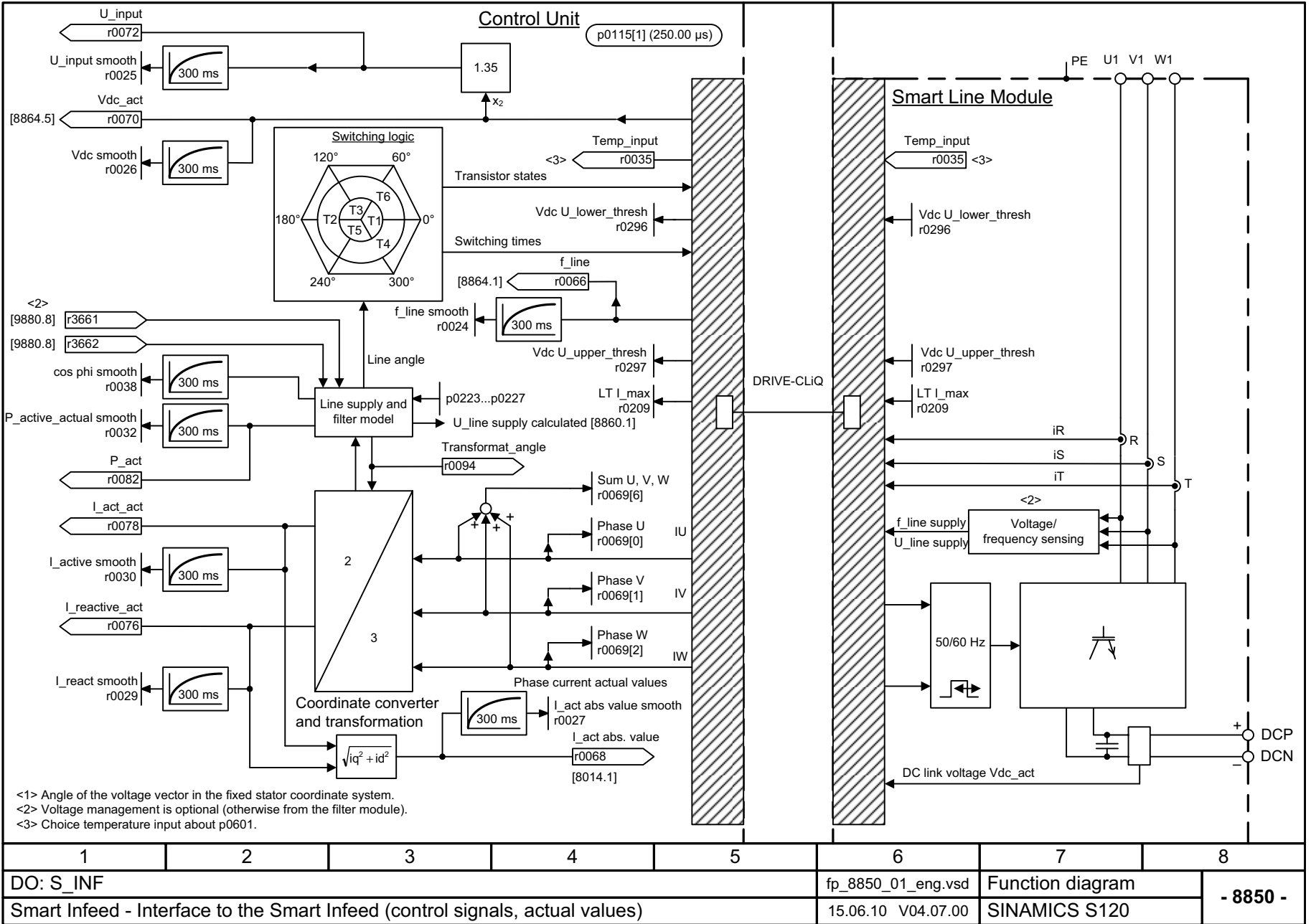
Fig. 3-313 8850 – Interface to the Smart Infeed (control signals, actual values)
