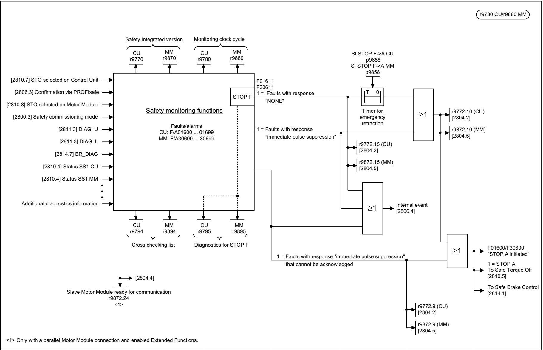
Fig. 3-110 2802 – Monitoring functions and faults/alarms
