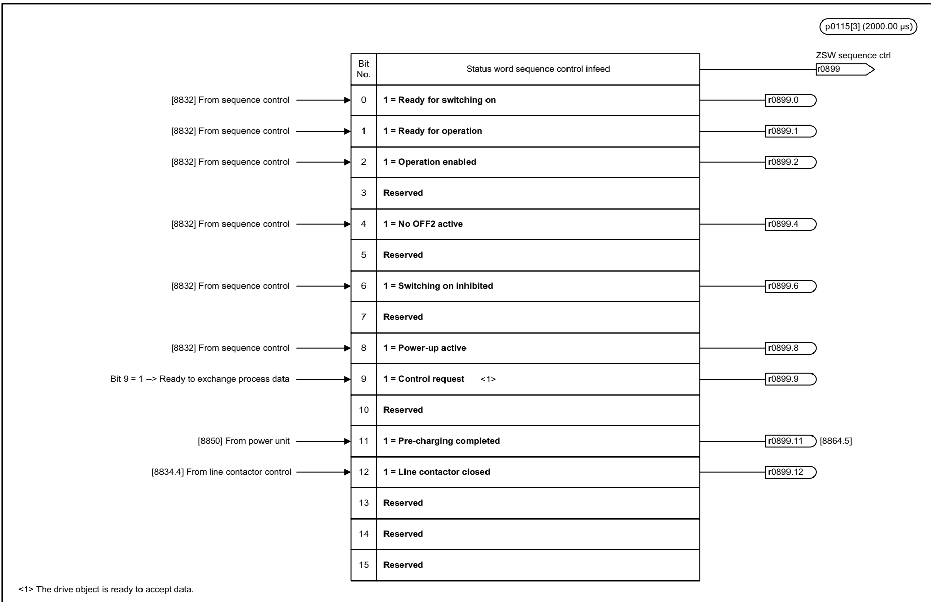
Fig. 3-309 8826 – Status word, sequence control infeed
