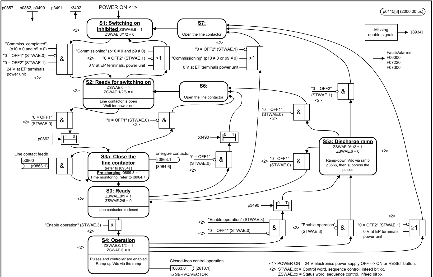
Fig. 3-320 8932 – Sequencer
