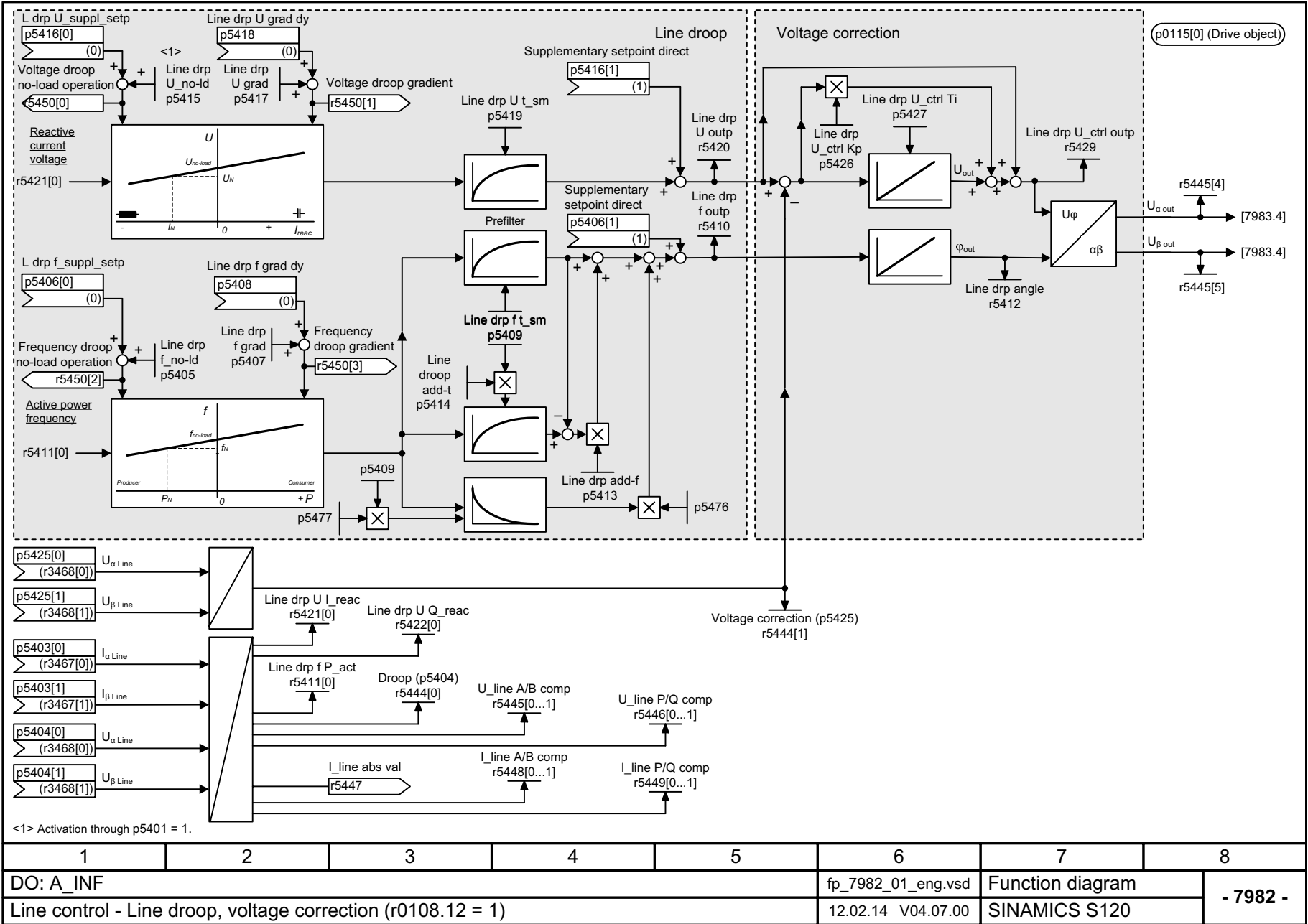
Fig. 3-264 7982 - Line droop, voltage correction (r0108.12 = 1)
