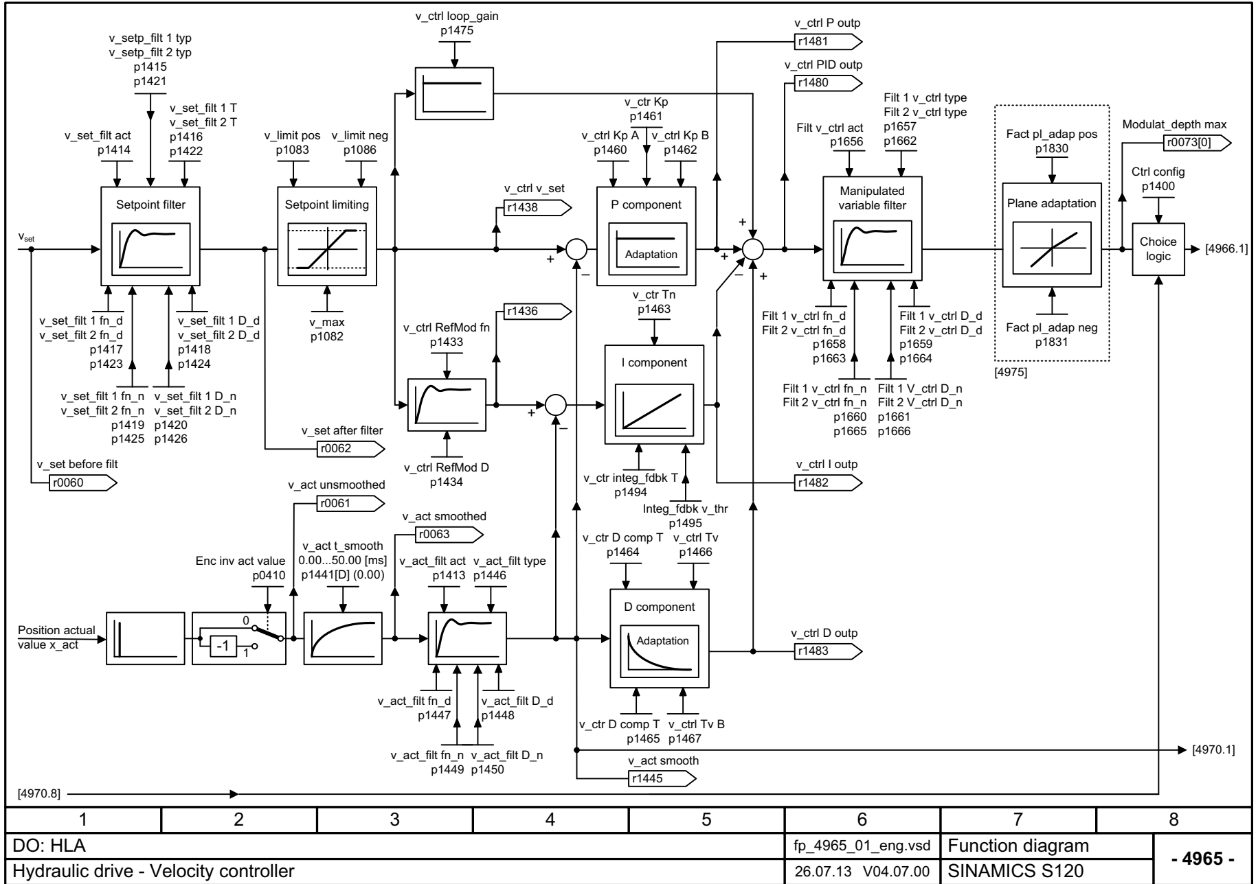
Fig. 3-187 4965 – Velocity controller
