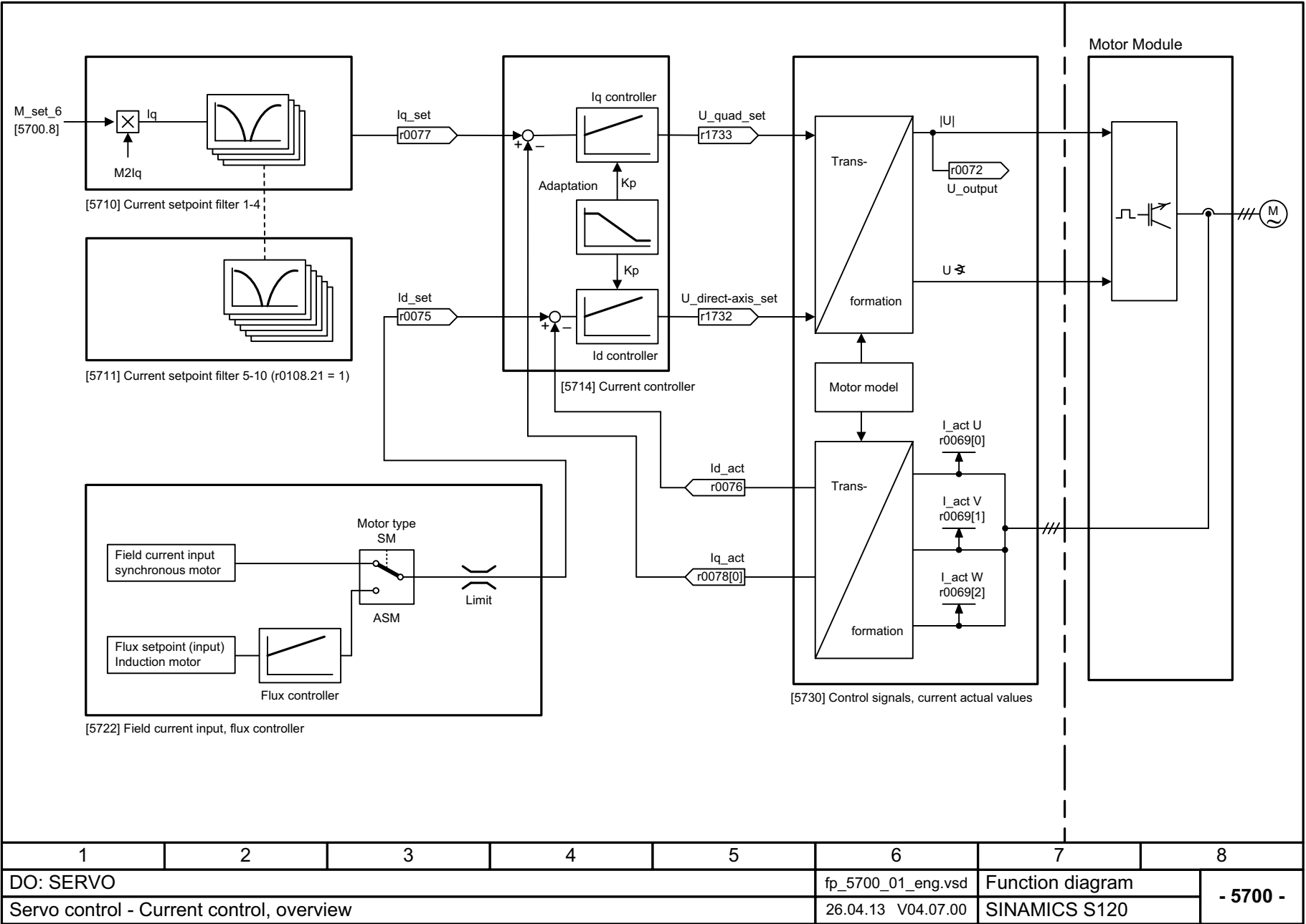
Fig. 3-2114 5700 – Current control, overview
