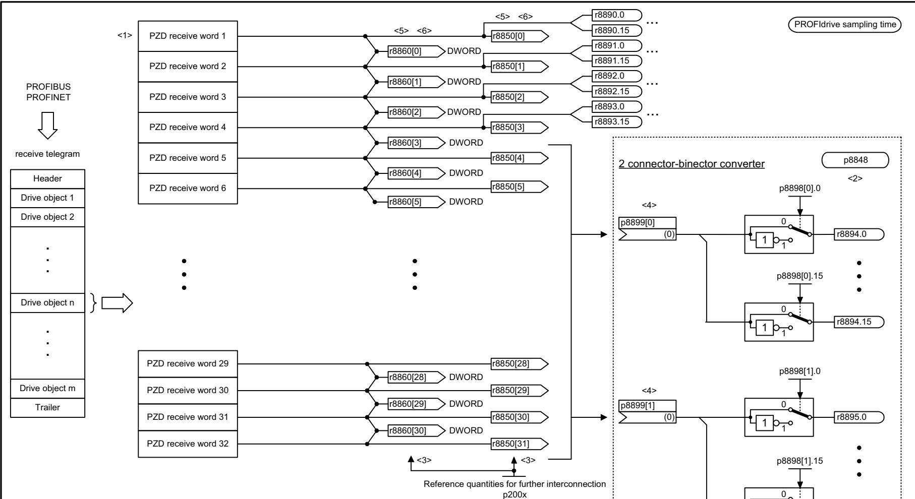
Fig. 3-80 2485 – IF2 receive telegram, free interconnection
