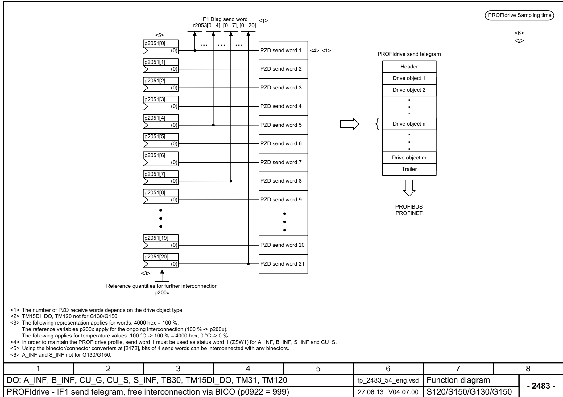
Fig. 3-79 2483 – IF1 send telegram, free interconnection via BICO (p0922 = 999)
