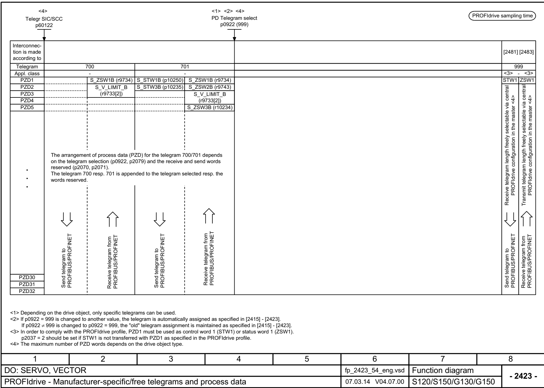
Fig. 3-40 2423 – Manufacturer-specific/free telegrams and process data
