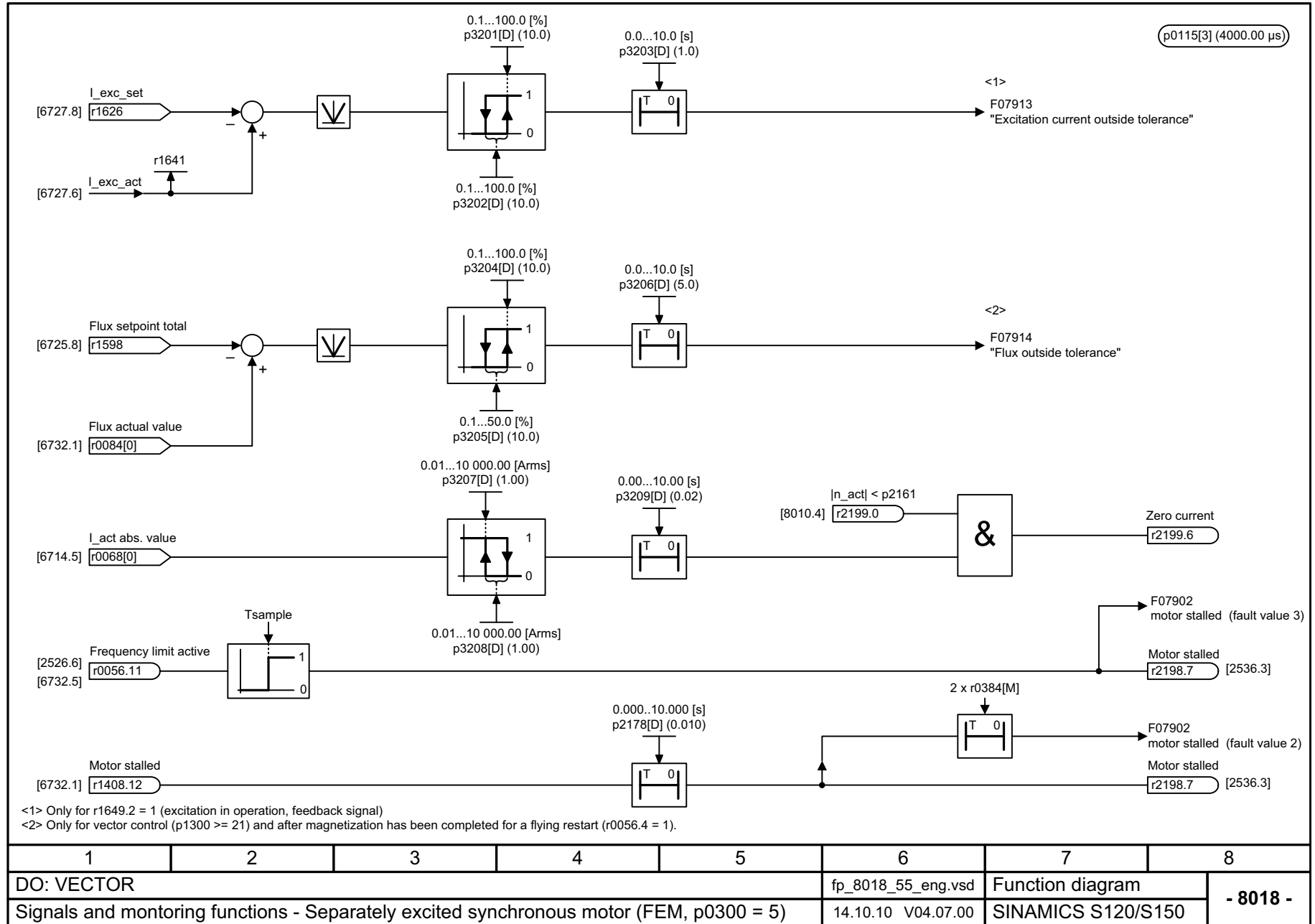
Fig. 3-288 8018 – Separately excited synchronous motor (FEM; p0300 = 5)
