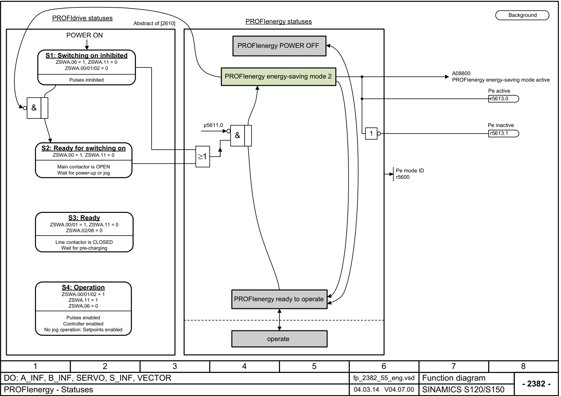
Fig. 3-31 2382 – States
