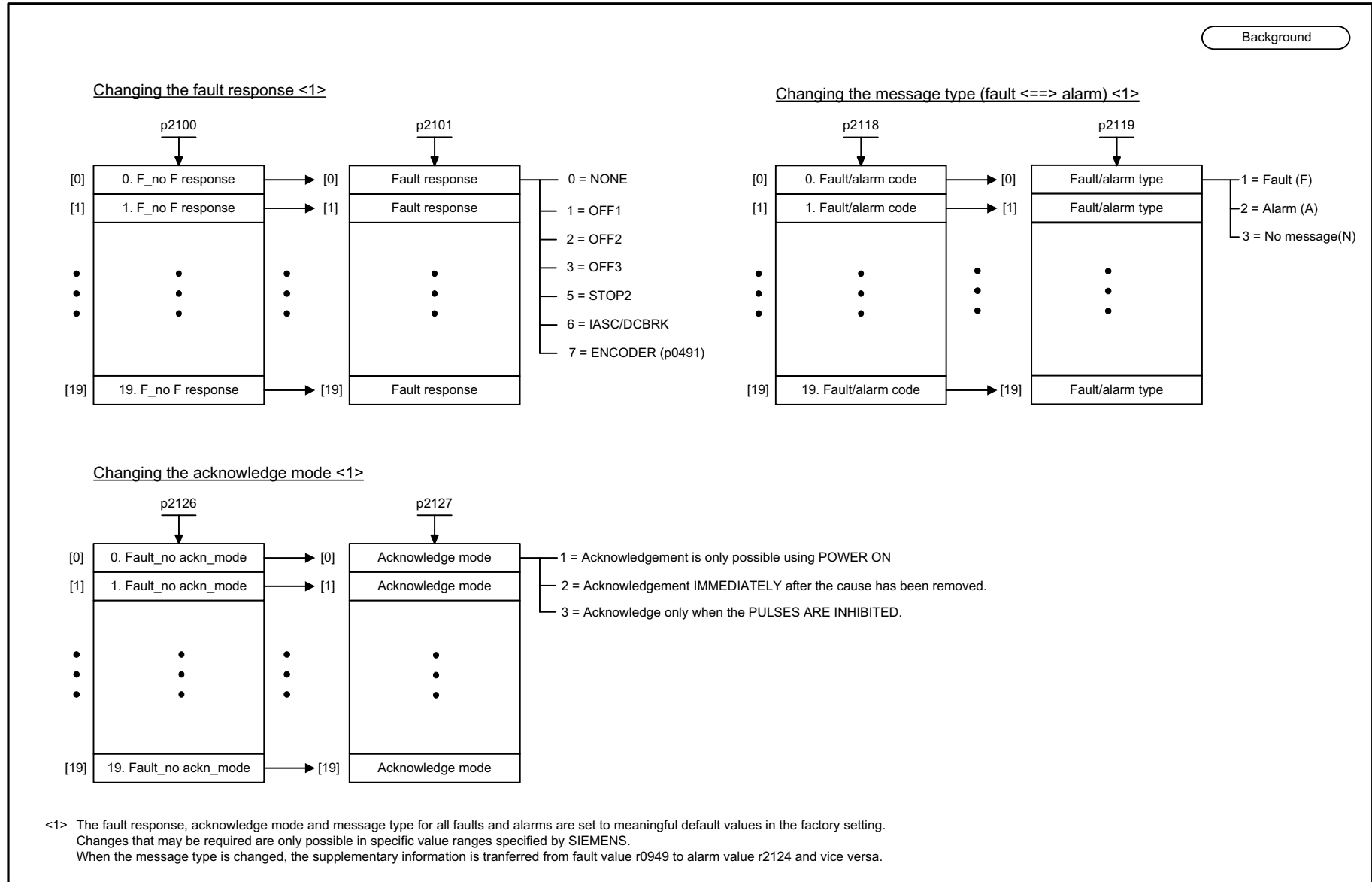
Fig. 3-293 8075 – Faults/alarms configuration
