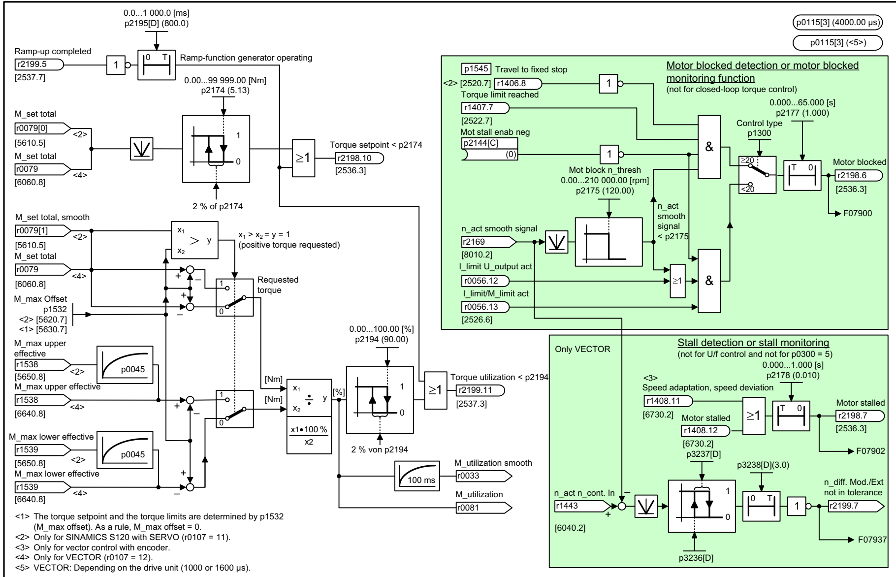
Fig. 3-283 8012 - Torque signals, motor blocked/stalled
