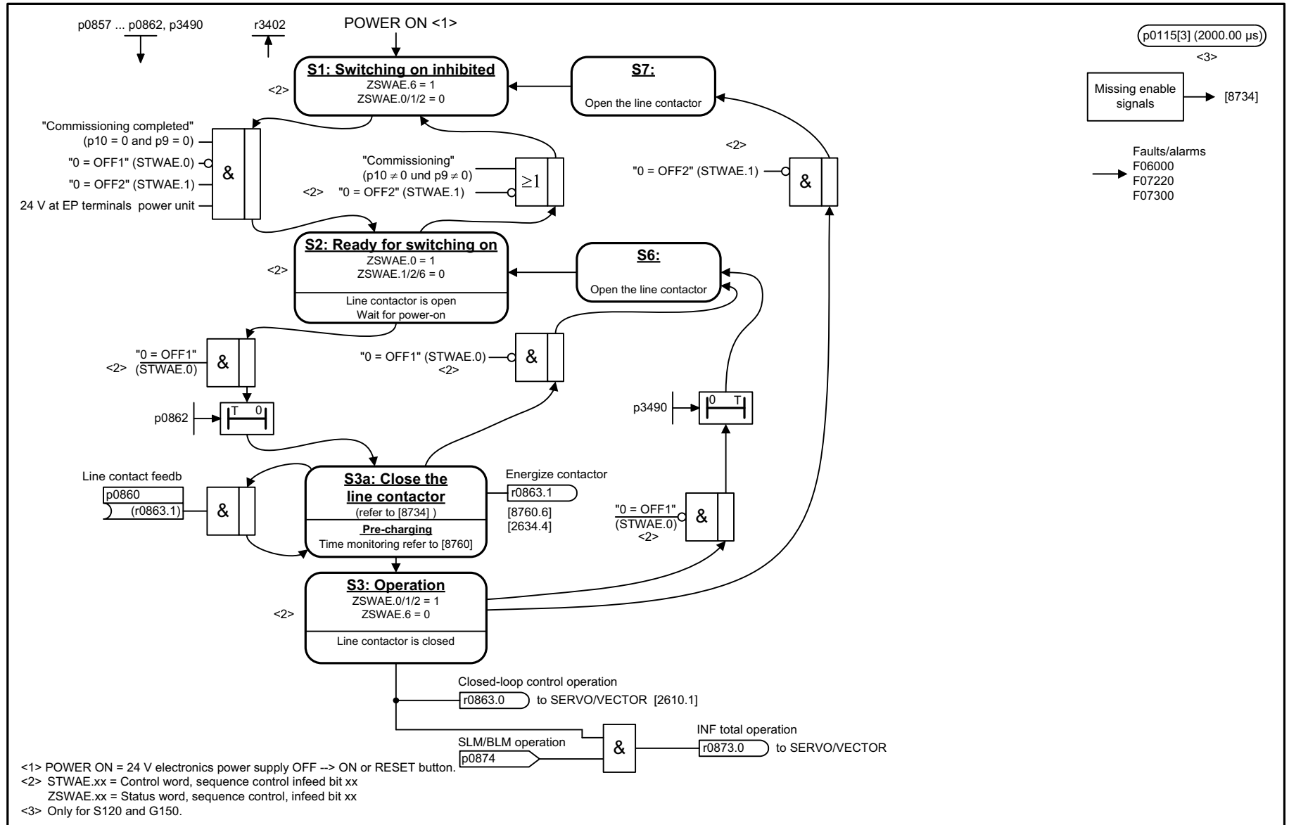
Fig. 3-303 8732 – Sequencer
