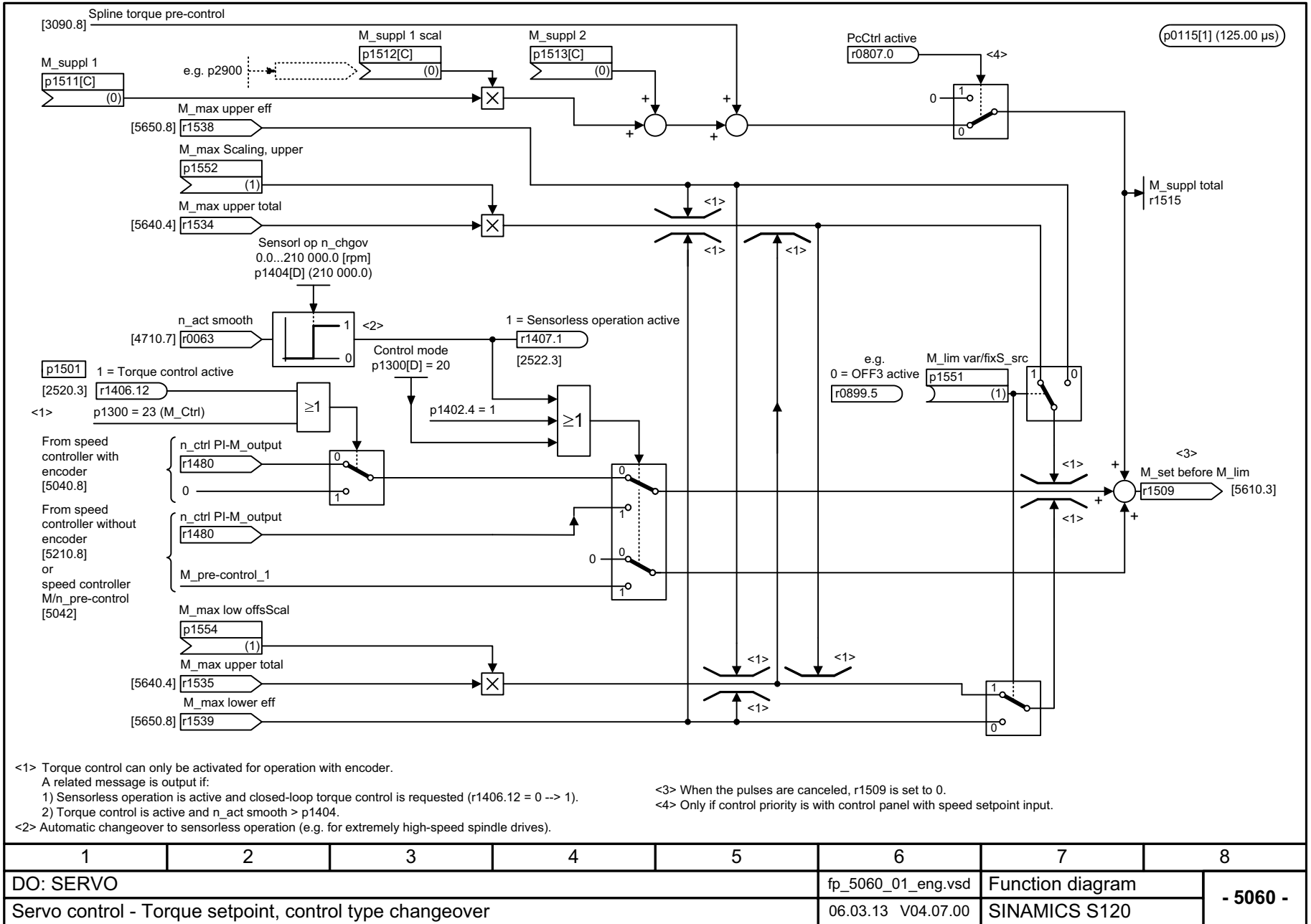
Fig. 3-203 5060 – Torque setpoint, control type changeover
